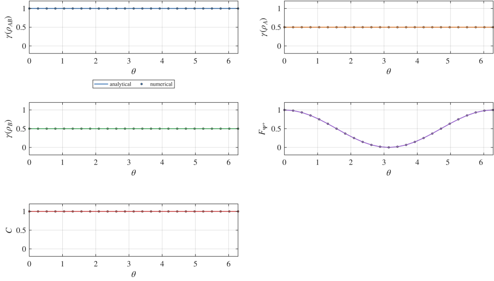
Figure 5.2: State-characterization quantities for the phase-evolved state. Global purity and concurrence remain constant, while fidelity varies with the relative phase \theta .
