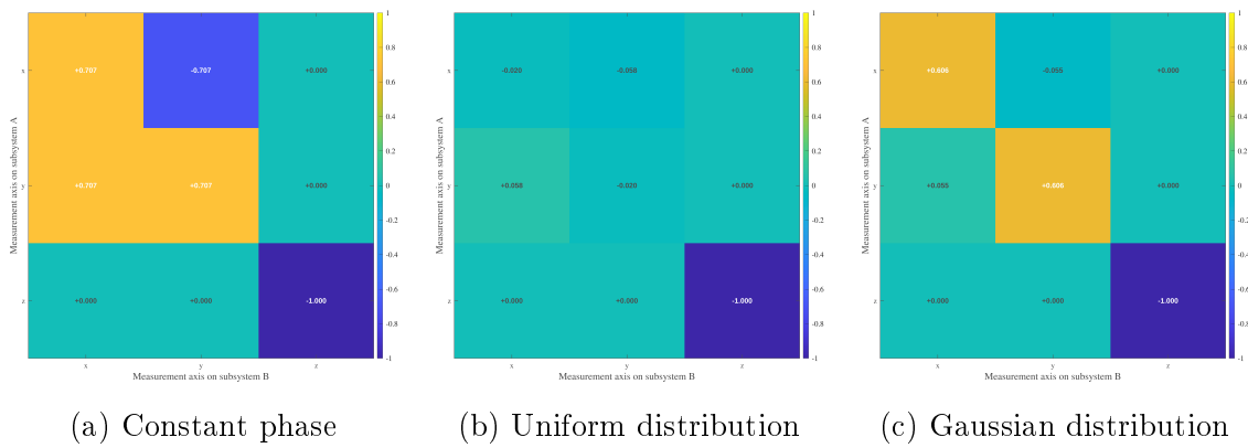
Figure 5.7: Correlation tensor snapshots for different phase distributions. Random phase averaging suppresses transverse coherence, progressively reducing the off-diagonal tensor components, while the longitudinal correlation T_{zz} = -1 remains invariant.
