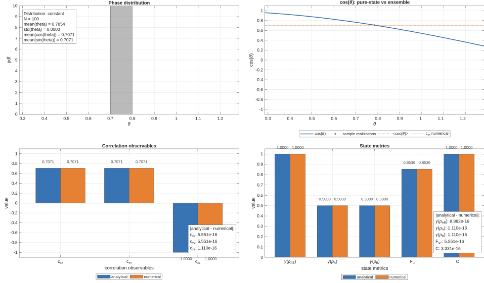
Figure 5.4: Constant phase distribution: the ensemble reduces to a deterministic realization and concurrence remains maximal.
