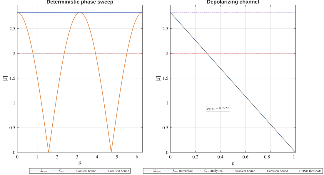
Figure 5.10: CHSH behavior under deterministic phase evolution and depolarizing noise. The left panel shows |S_{\text{fixed}}| and S_{\text{max}} as functions of the phase parameter \theta . The right panel shows the corresponding quantities as functions of the depolarizing parameter p . The red dotted line indicates the classical CHSH bound |S| = 2 , while the purple dotted line corresponds to the Tsirelson bound 2\sqrt{2} .
