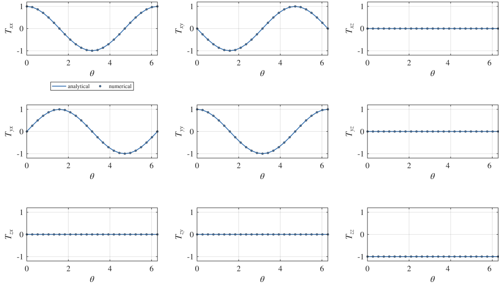
Figure 5.3: Full correlation tensor T_{ij}(\theta) for the phase-evolved state. The off-diagonal tensor components reveal the rotation of the correlation structure in the transverse plane.
