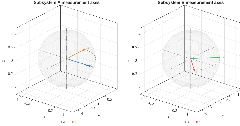
Figure 5.9: Fixed CHSH measurement axes represented on the Bloch spheres of subsystems A and B . The analyzer directions define the fixed laboratory configuration used to evaluate S_{\text{fixed}} .
