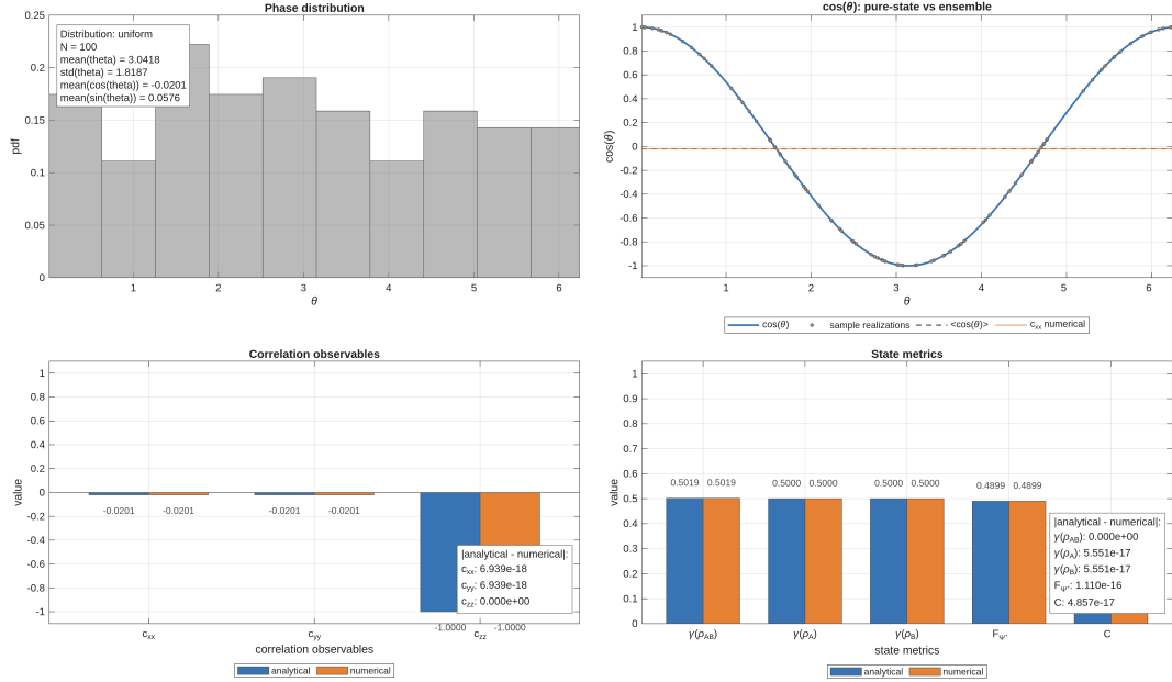
Figure 5.5: Uniform phase distribution: transverse correlations vanish, fidelity decreases, and concurrence tends to zero.
