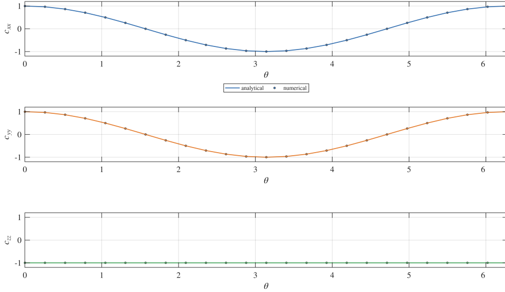
Figure 5.1: Numerical and analytical comparison for the correlation observables c_{xx} , c_{yy} , and c_{zz} . The agreement validates the implementation of the reduced phase model.
