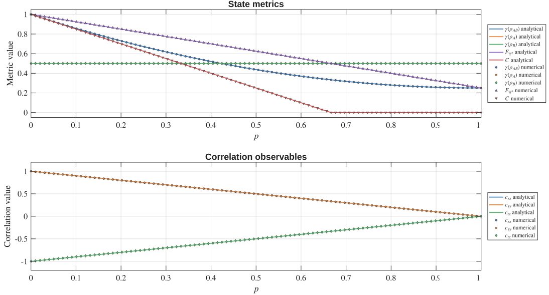
Figure 5.8: Numerical and analytical behavior of purity, fidelity, concurrence, and correlations under the depolarizing channel. Agreement is exact up to numerical precision.
