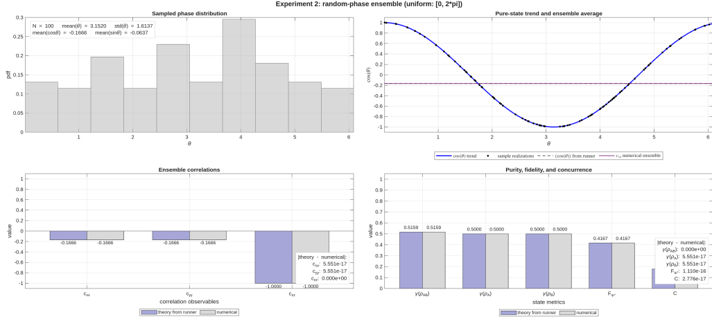
Figure 4: Summary of Experiment 2 for a uniform phase distribution. Phase averaging suppresses transverse correlations, reduces fidelity, and drives concurrence to zero.
