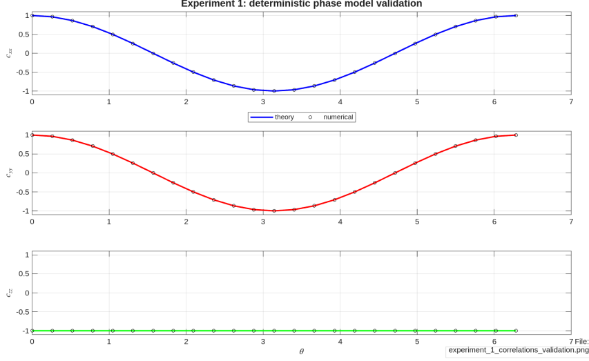
Figure 1: Comparison between numerical simulation and analytical predictions for the correlation observables c_{xx} , c_{yy} , and c_{zz} as functions of the relative phase \theta . The agreement confirms the correctness of the reduced phase model implementation.
