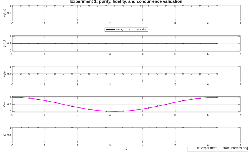
Figure 2: Numerical and analytical comparison of state-characterization quantities for the phase-evolved state. The figure shows global purity \gamma(\rho_{AB}) , reduced purities \gamma(\rho_A) and \gamma(\rho_B) , fidelity with respect to |\Psi^+\rangle , and concurrence. While fidelity varies with \theta , concurrence remains constant and equal to one.
