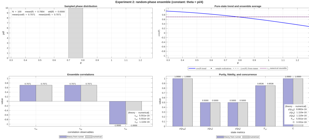
Figure 3: Summary of Experiment 2 for a constant phase distribution. The ensemble reduces to a single deterministic realization, and concurrence remains equal to one.
