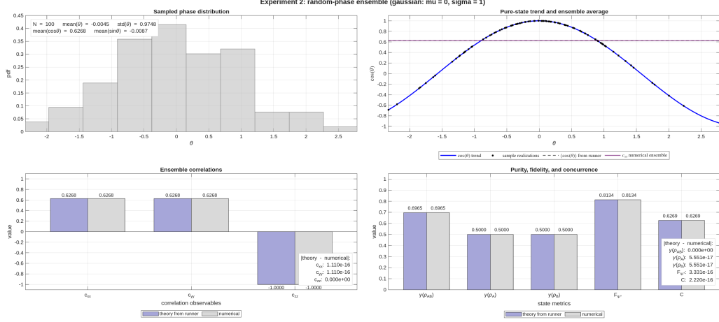
Figure 5: Summary of Experiment 2 for a Gaussian phase distribution. Residual coherence depends on the phase variance, leading to intermediate values of concurrence.
