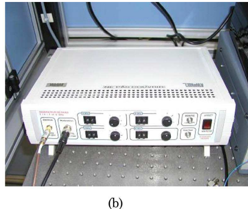
Fig. 7. (Color online) (a) Nonsinusoidal phase modulation scheme: the harmonic combination and phase control is performed directly with the HF signal. Optical components remain the same. (b) HF multiharmonic generator at 2–4–6 GHz used in our different setups.
