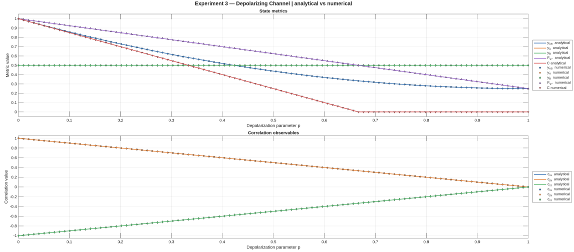
Figure 8: Numerical and analytical behavior of purity, fidelity, concurrence, and correlations under the depolarizing channel. Agreement is exact up to numerical precision.
