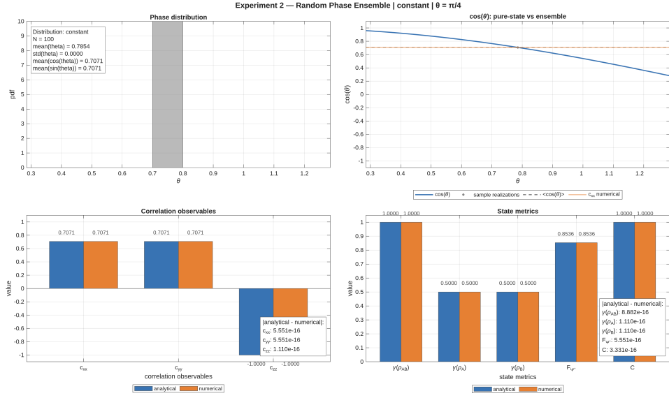
Figure 4: Constant phase distribution: the ensemble reduces to a deterministic realization and concurrence remains maximal.
