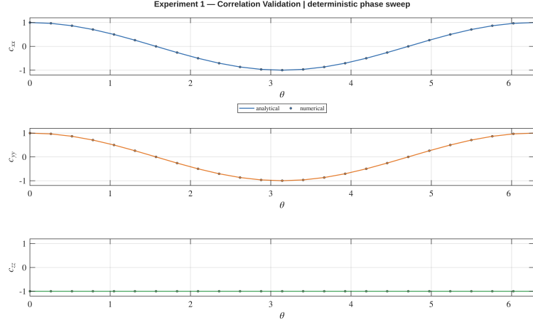
Figure 1: Numerical and analytical comparison for the correlation observables c_{xx} , c_{yy} , and c_{zz} . The agreement validates the implementation of the reduced phase model.
