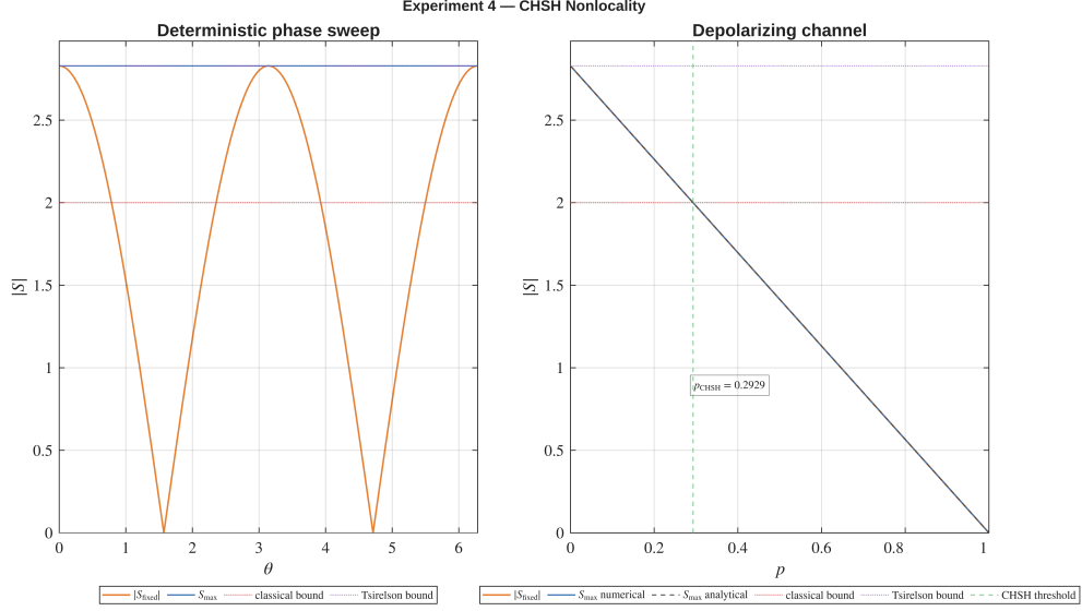
Figure 10: CHSH behavior under deterministic phase evolution and depolarizing noise. The left panel shows |S_{\text{fixed}}| and S_{\text{max}} as functions of the phase \theta . The right panel shows the corresponding quantities as functions of the depolarizing parameter p . The red dotted line is the classical CHSH bound |S| = 2 , while the purple dotted line is the Tsirelson bound 2\sqrt{2} .
