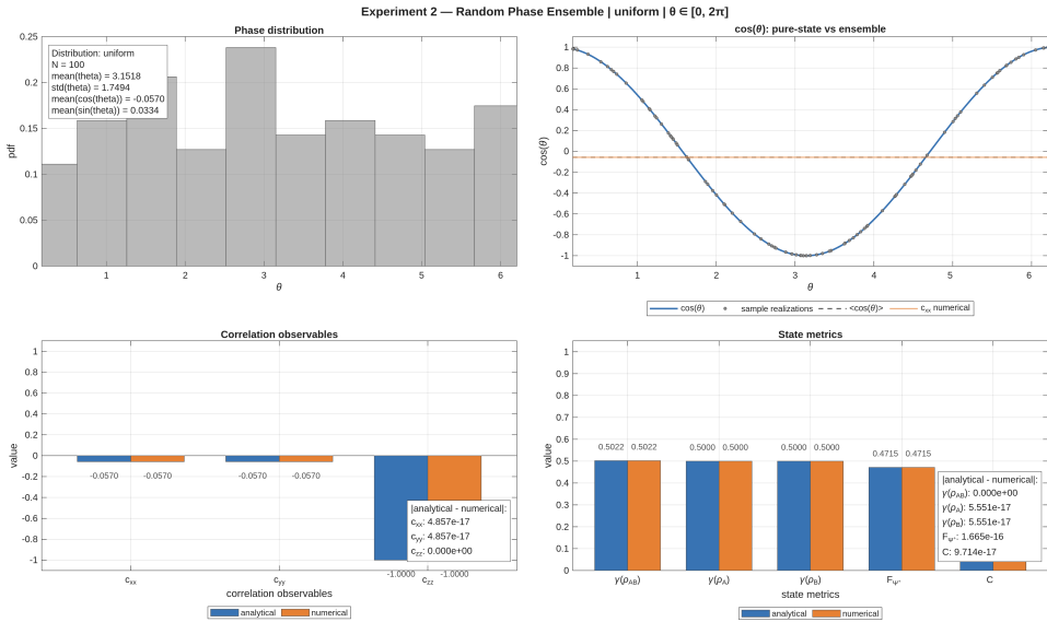
Figure 5: Uniform phase distribution: transverse correlations vanish, fidelity decreases, and concurrence tends to zero.
