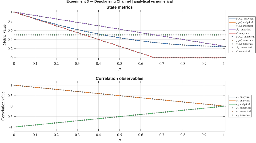
Figure 8: Numerical and analytical behavior of purity, fidelity, concurrence, and correlations under the depolarizing channel. Agreement is exact up to numerical precision.
