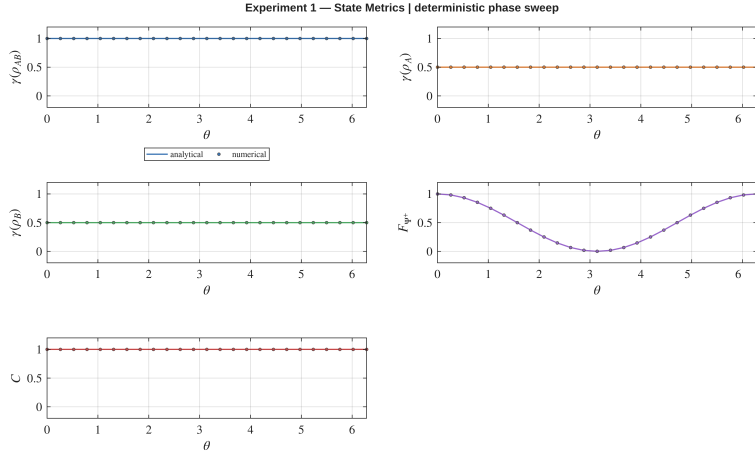
Figure 2: State-characterization quantities for the phase-evolved state. Global purity and concurrence remain constant, while fidelity varies with the relative phase \theta .
