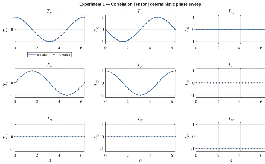
Figure 3: Full correlation tensor T_{ij}(\theta) for the phase-evolved state. The off-diagonal components T_{xy} and T_{yx} reveal the rotation of the correlation structure in the transverse plane.
