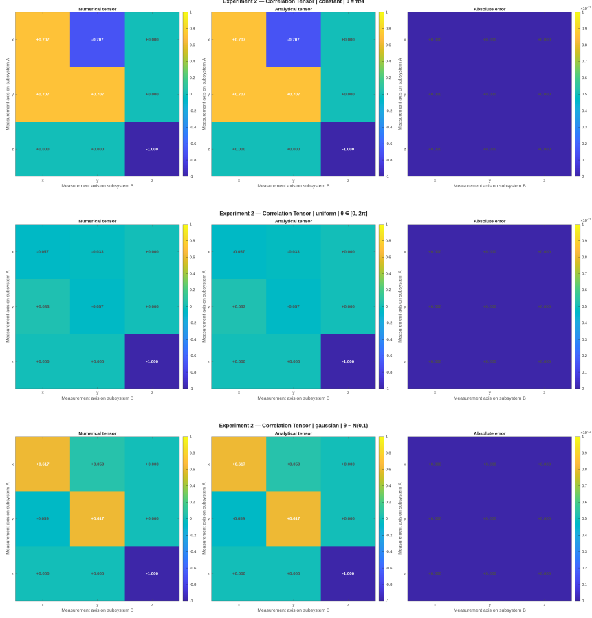
Figure 7: Correlation tensor snapshots for the three random-phase ensemble cases: constant, uniform, and Gaussian phase distributions. The tensor visualization shows that random phase averaging mainly suppresses the transverse coherence terms, while the longitudinal anti-correlation T_{zz} remains fixed at -1 .
