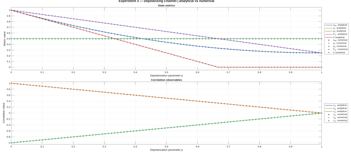
Figure 8: Experiment 3: numerical and analytical behavior of state metrics and Pauli correlations under the two-qubit depolarizing channel applied to the Bell state |\Psi^+\rangle . The agreement is exact up to numerical precision.
