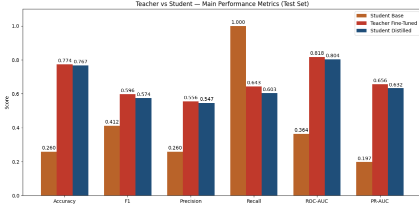
Figure 3: Bar charts that compares the metrics of base student, distilled student and fine-tuned teacher
