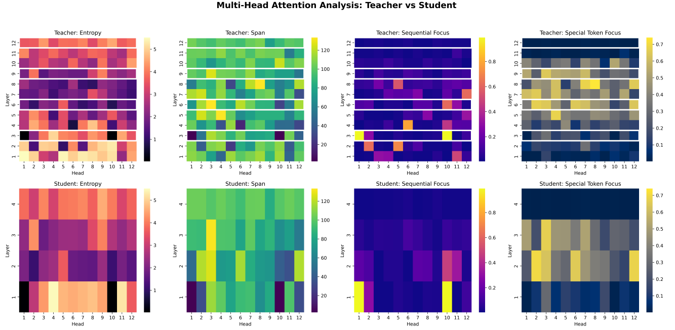
Figure 6: Multi-head Attention analysis through heatmaps
