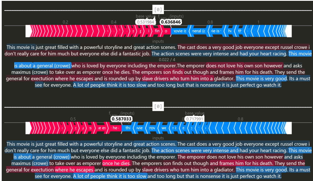
Figure 7: SHAP-based analysis (Label 0 = Spoiler; Label 1 = No Spoiler)
