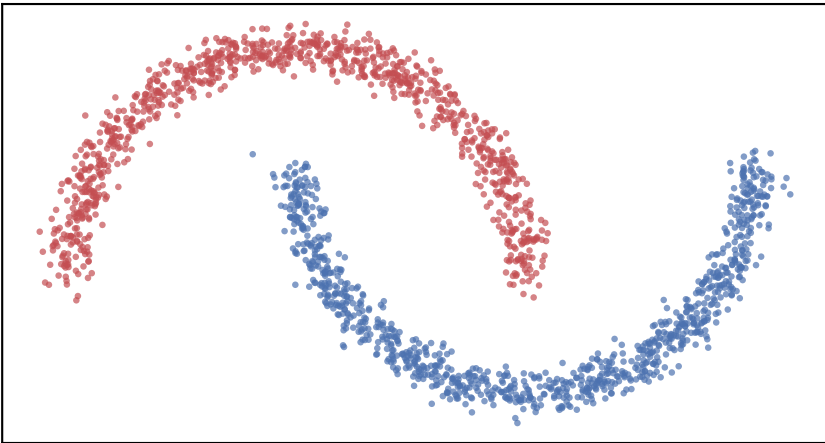
Moons, \eta = 0
