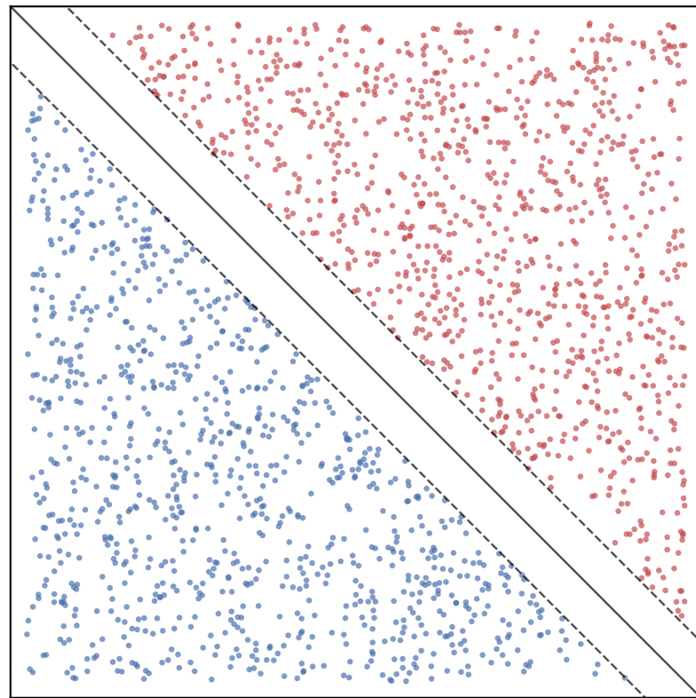
Diagonal, \gamma = 0.12
