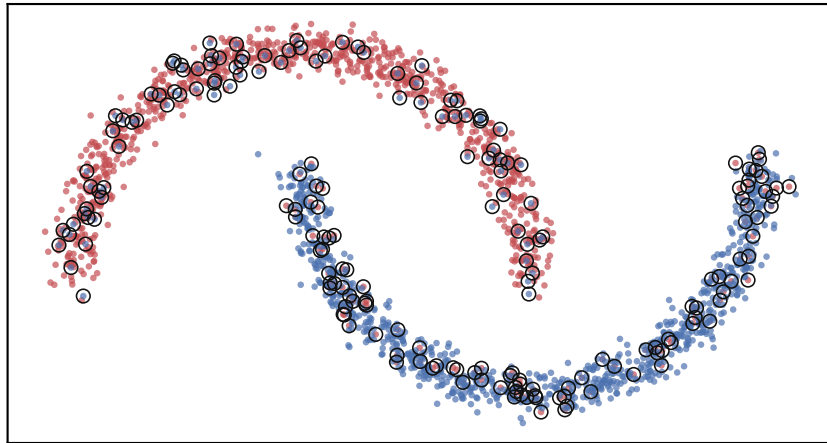
Moons, \eta = 0.10
