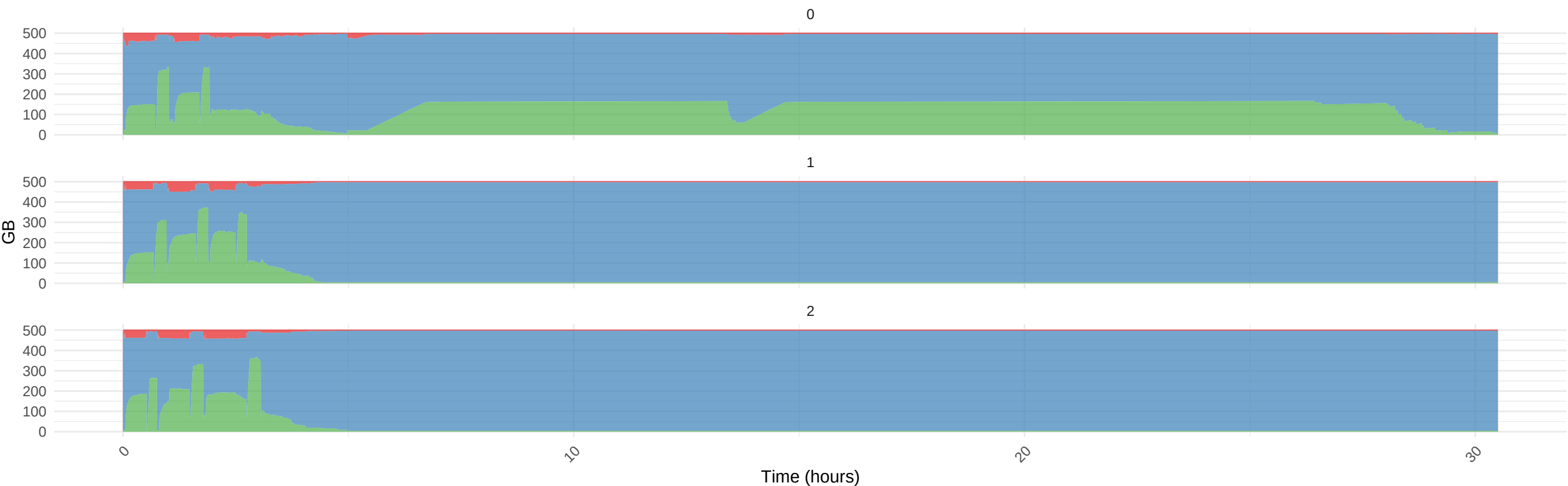
Memory Usage Over Time (GB)
