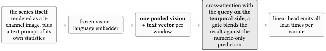
Figure 4: Time-VLM [2]. The imagery is manufactured from the numeric input rather than observed, and the pooled multimodal vector serves as keys and values for a query formed from the temporal state.
