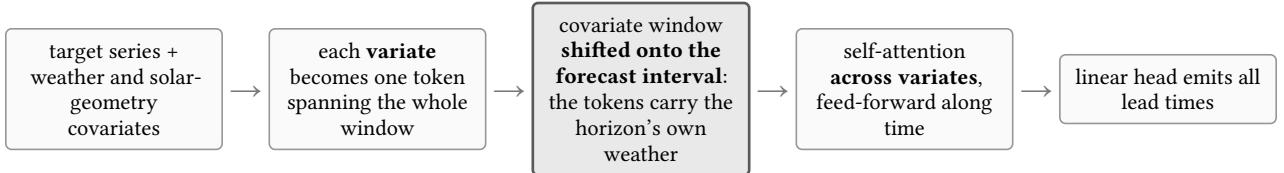
Figure 5: iTransformer [9] with covariates. Inverting the transformer’s axes makes each variate a token; with the covariate window shifted forward, the exogenous channel is already aligned to the lead times being predicted.
