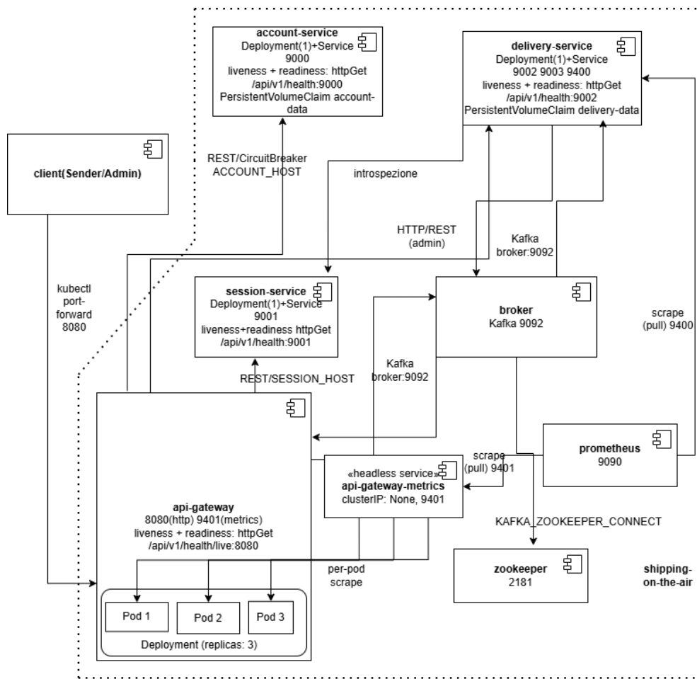
Deployment Kubernetes
