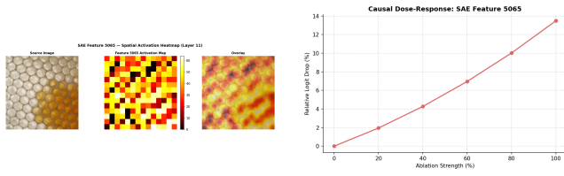
Figure 2: Feature 5065. Left: spatial activation heatmap showing selective activation on coherent regions. Right: dose-response curve—monotonically increasing logit drop as ablation strength goes from 0 to 1.
