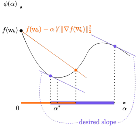
Figure 2. Wolfe conditions
