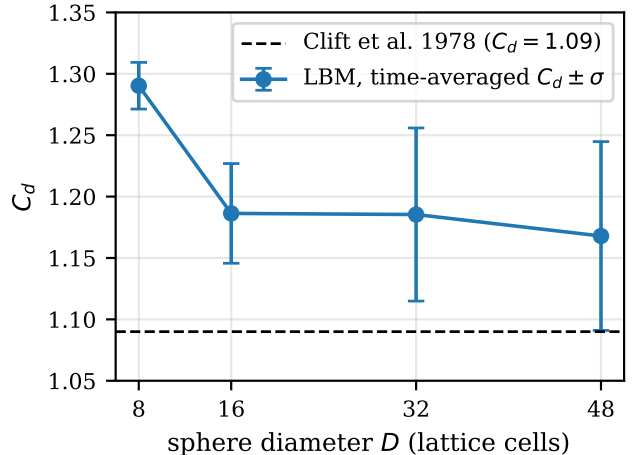
Figure 2: Sphere C_d grid convergence at Re = 100 . Points: LBM time-averaged C_d with \pm\sigma error bars (Table 2). Dashed line: Clift correlation. The residual \sim 7\% gap at the finest grid is consistent with blockage ( D/L_y = 0.25 ) and the un-tuned MRT relaxation rates.
