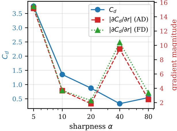
Figure 4: Sensitivity of C_d (blue, left axis) and |\partial C_d / \partial r| (red/green, right axis) to the sigmoid sharpness \alpha at r = 0.5 on the 96 \times 48 \times 48 grid. The gradient sign is stable across a decade in \alpha ; magnitudes are not. AD and FD track each other closely throughout.
