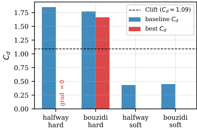
(a) baseline vs best C_d
