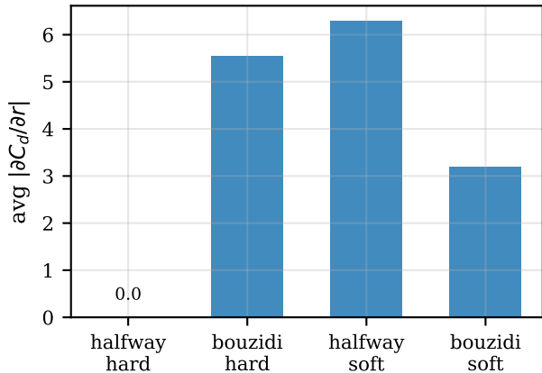
(b) average gradient magnitude
