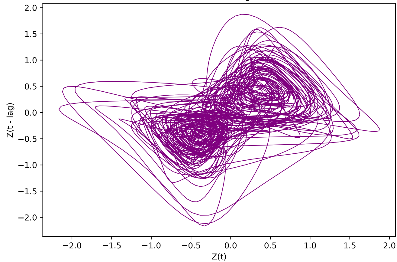
Attractor reconstruction (Test Phase) Z(t) vs Z(t-lag)
