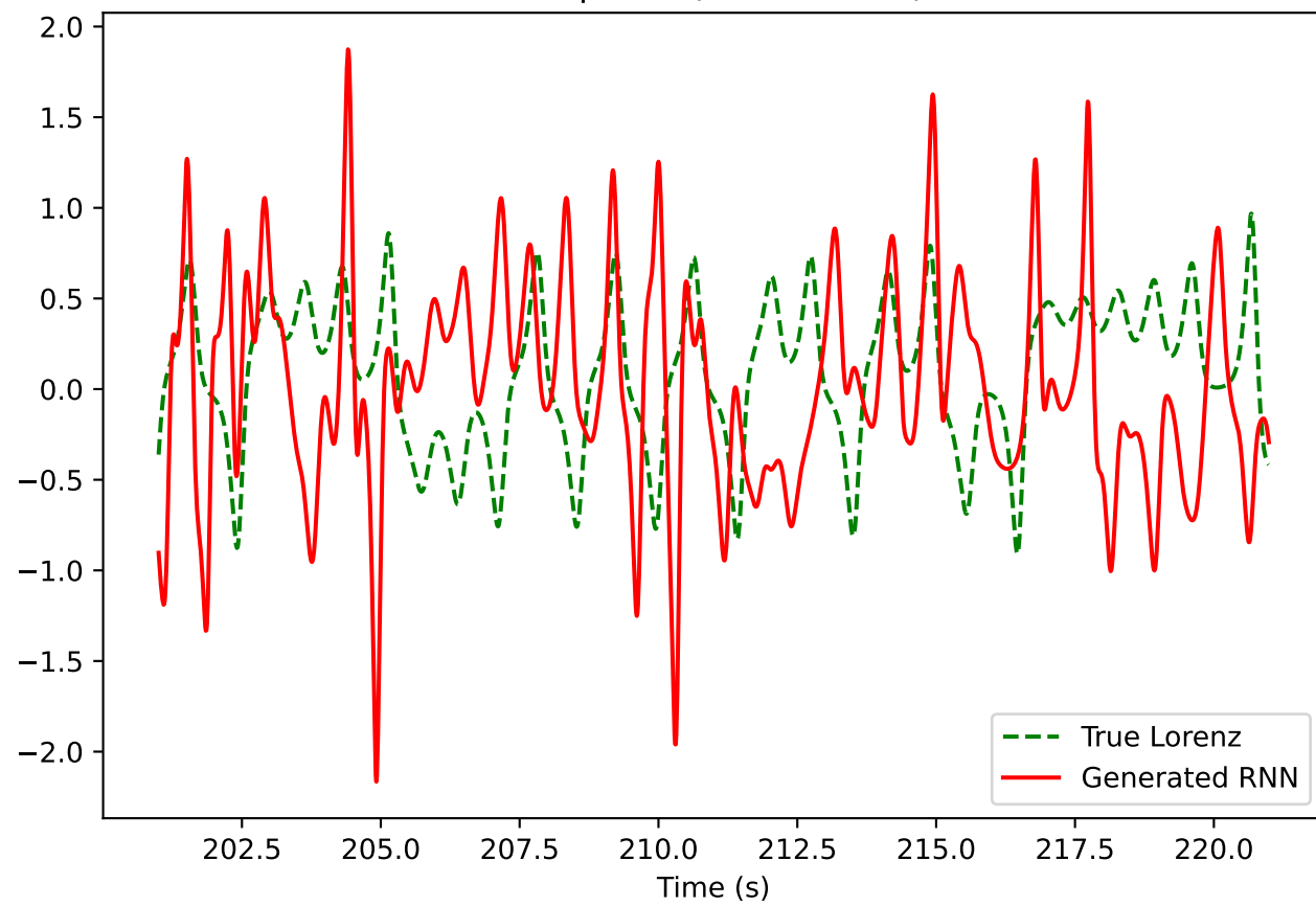
Test phase (autonomous)
