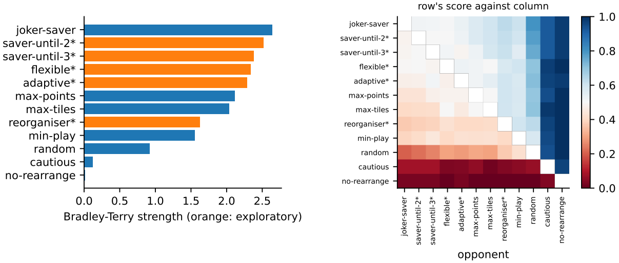
Figure 5: Extended league. Left: Bradley-Terry strength (orange: exploratory strategies). Right: score of the row strategy against the column strategy (80 seeds, both seats).
