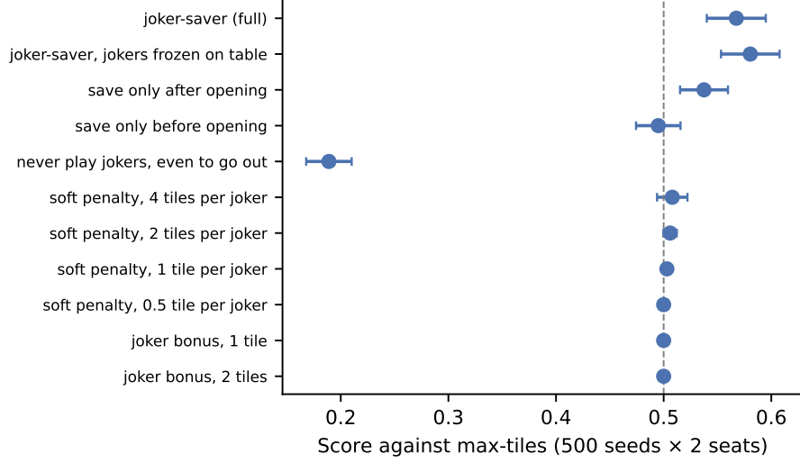
Figure 2: Mechanism experiments (mean \pm 95% CI).
