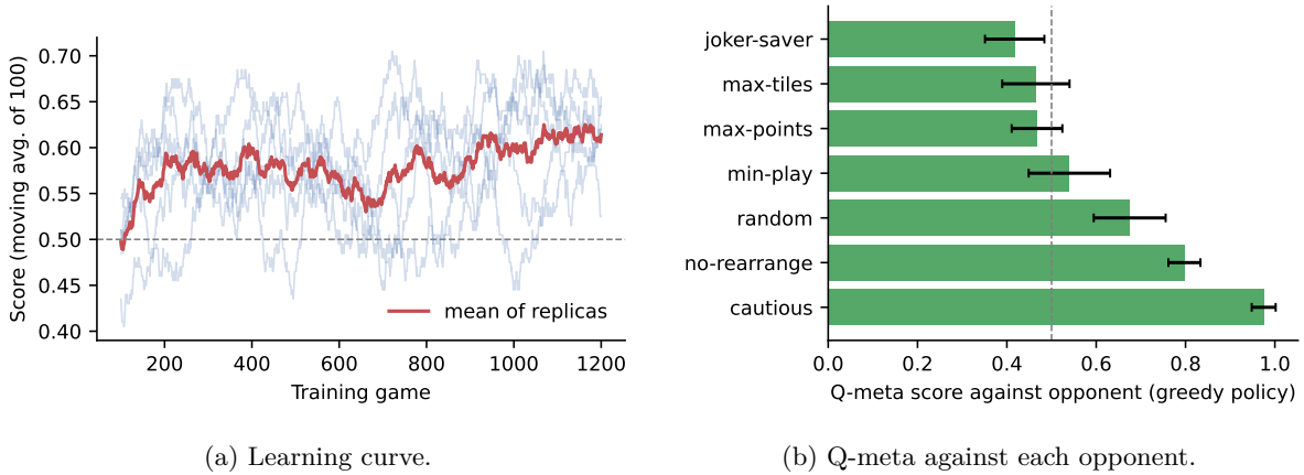
Figure 8: Q-meta training and evaluation (5 replicas).
