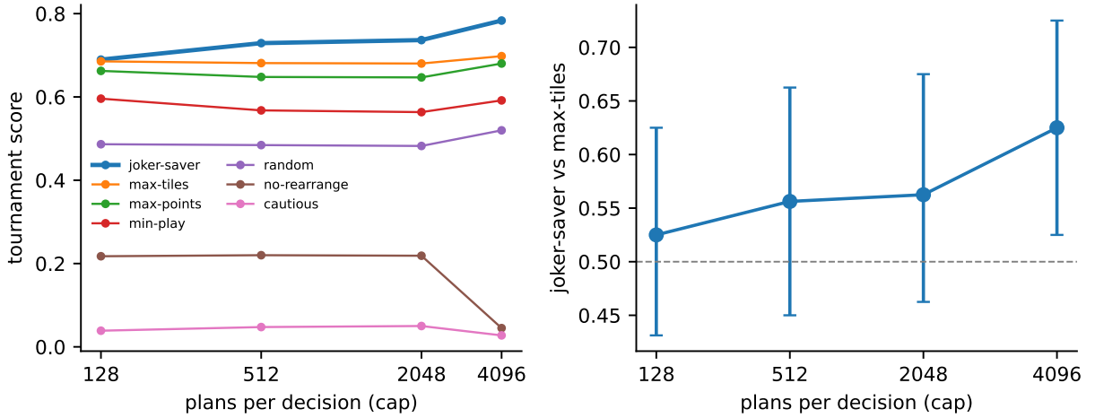
Figure 3: Left: tournament score of each strategy by rearrangement cap. Right: joker-saver against max-tiles with the 95% bootstrap interval over 40 seeds.
