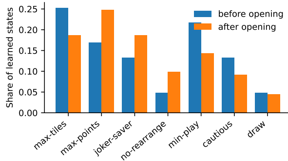
Figure 9: Share of learned states where each strategy has the highest Q-value, by opening status.
