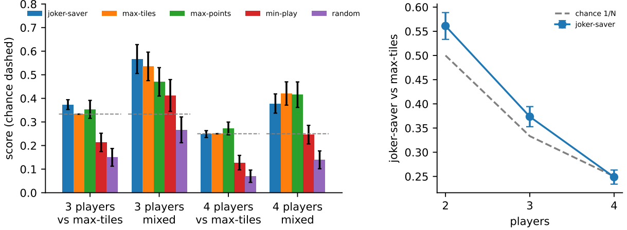
Figure 4: Left: score of five strategies at three- and four-player tables (dashed: chance 1/N ). Right: joker-saver against max-tiles as the number of players grows ( \pm 1.96 standard errors over seeds).
