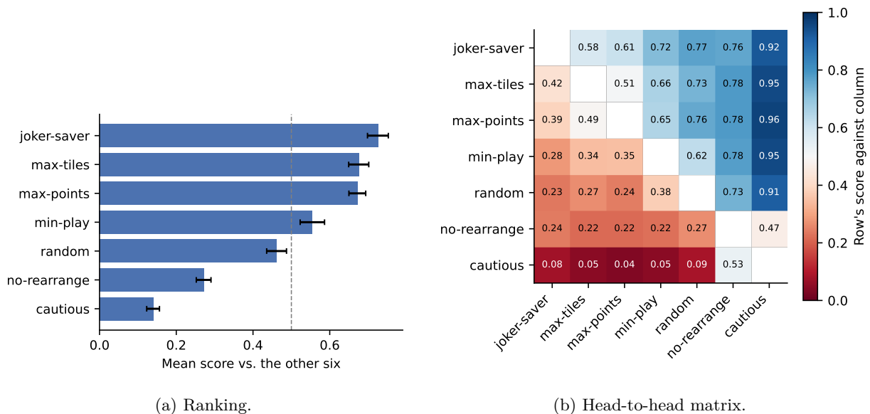
Figure 1: Paired round-robin (3,360 games); score: win = 1, draw = 0.5.
