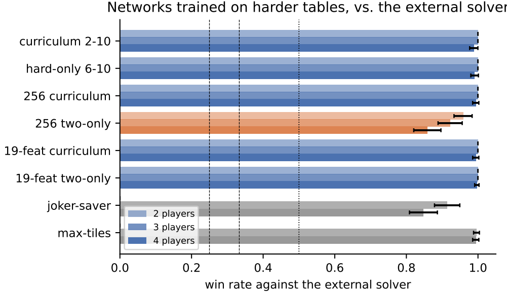
Figure 13: Networks trained on harder or larger settings, played against the external solver ( N - 1 copies in the field; shade = table size). All crush it except the 256-unit network trained only at two players; the joker-saver also trails at four players.
