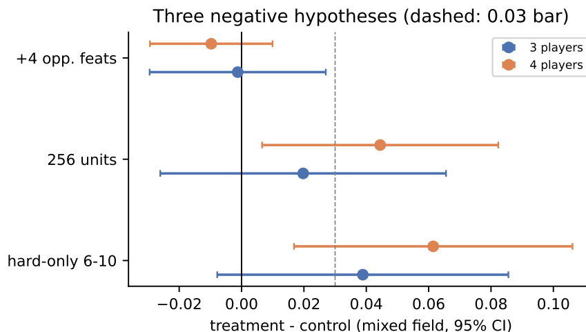
Figure 11: Three negative hypotheses, development seeds: treatment minus the two-player control in the mixed field (95% CI). None clears the pre-set 0.03 bar with a positive interval at both table sizes.
