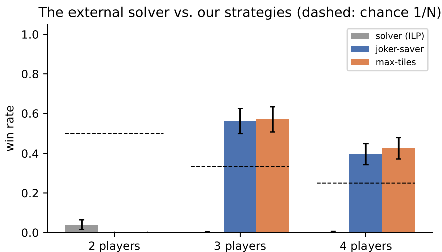
Figure 12: The external ILP solver, wrapped as a greedy player, against our two best heuristics (dashed: chance 1/N ). It wins almost nothing.
