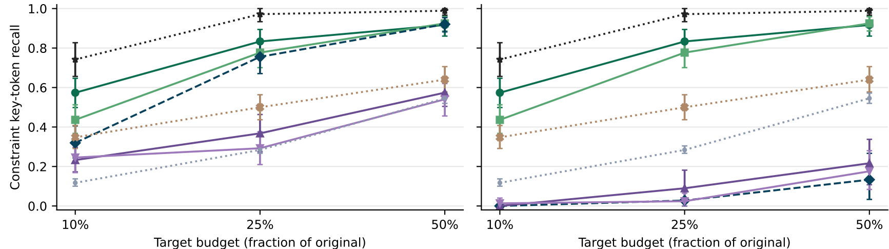
(a) Paper metric: recall after truncation
