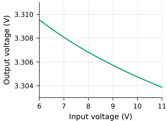
3.3 V mode, load 3.3 \Omega
