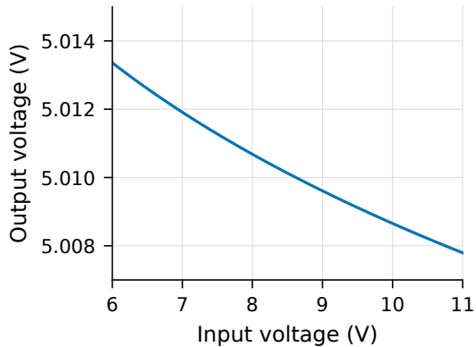
5 V mode, load 5 \Omega
