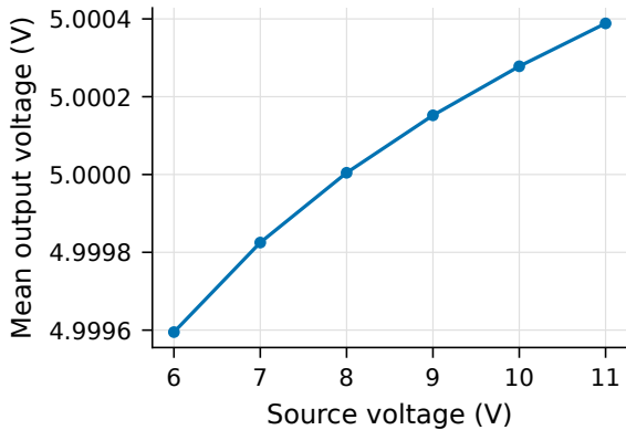
(a) 5 V mode, 5 \Omega load
