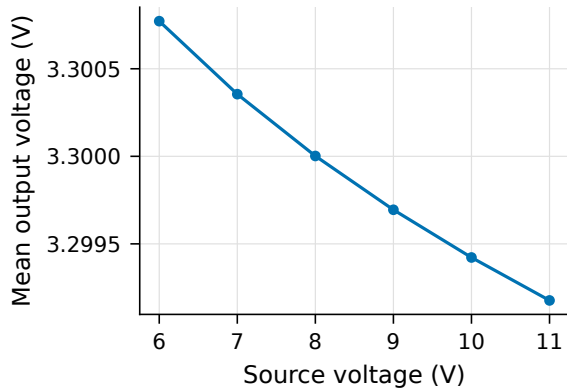
(b) 3.3 V mode, 3.3 \Omega load
