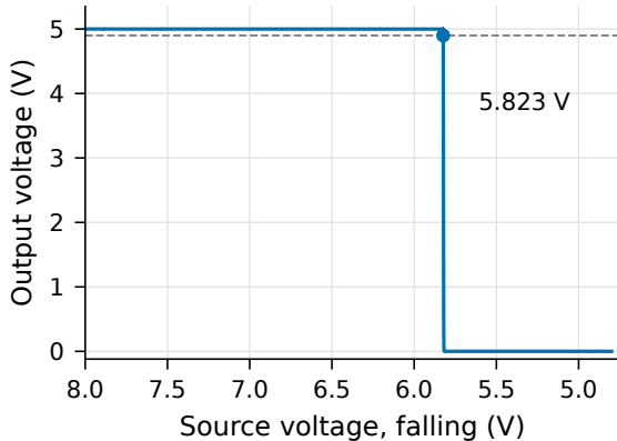
(a) 5 V mode
