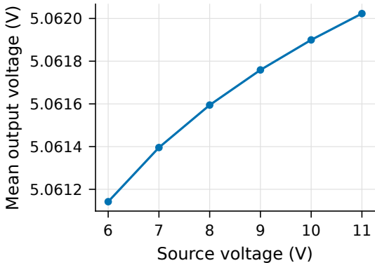
Full circuit, 5 \Omega load
