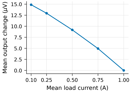
(a) 5 V mode
