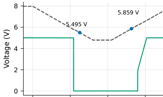
(a) Undervoltage cycle
