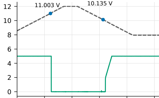
(b) Overvoltage cycle
