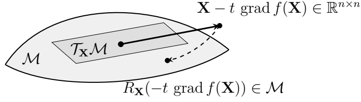
Figure 3: Illustration of a retraction. Starting from \mathbf{X} \in \mathcal{M} , a tangent step is taken along the negative Riemannian gradient in the tangent space \mathcal{T}_{\mathbf{X}}\mathcal{M} . Since the point \mathbf{X} - t \text{grad } f(\mathbf{X}) does not generally belong to the manifold, the retraction maps it back onto \mathcal{M} .
