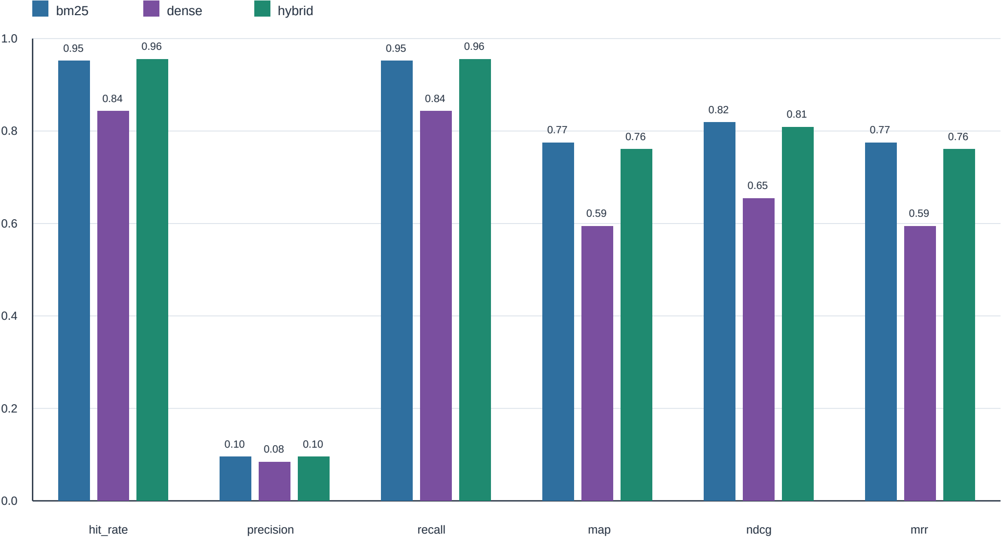
SciQ retrieval metrics at k=10
