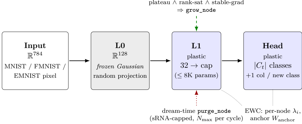
Figure 1: Base trioron architecture for chained-15. The frozen Gaussian L0 projection provides a stable code space for manifold replay (§3.6). The plastic L1 grows under the conjunction of loss-plateau, rank-saturation, and gradient-stability triggers up to a per-curriculum byte cap; the head grows one column per new class. Dream-time purge removes low-utility nodes, gated by the per-cycle event cap (§3.5.2). EWC anchors plus per-node plasticity \lambda_i pin prior-task knowledge on plastic layers.
