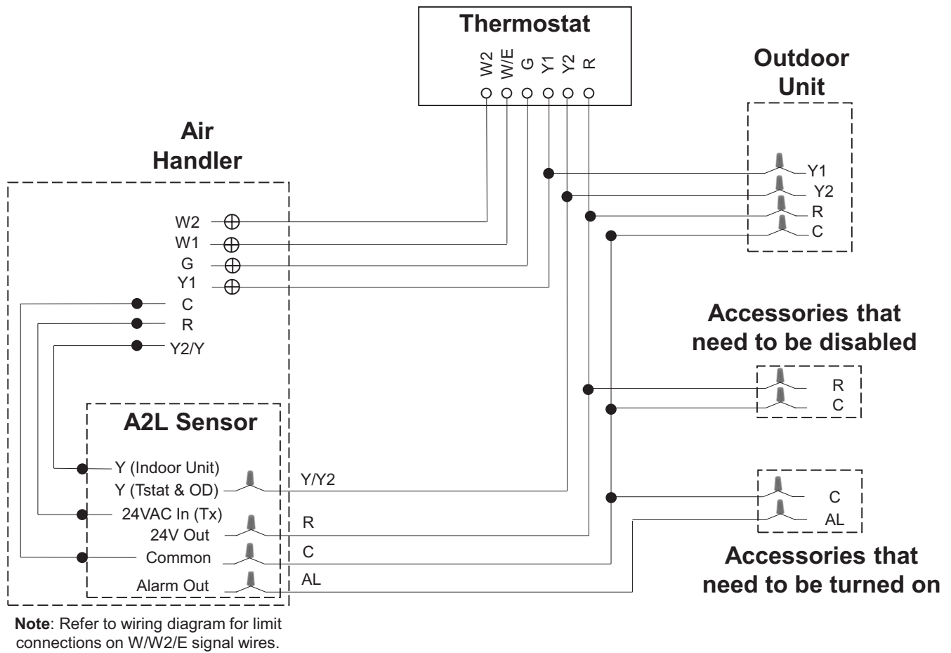
Figure 18. Typical two-stage air handler with two-stage air conditioner.
