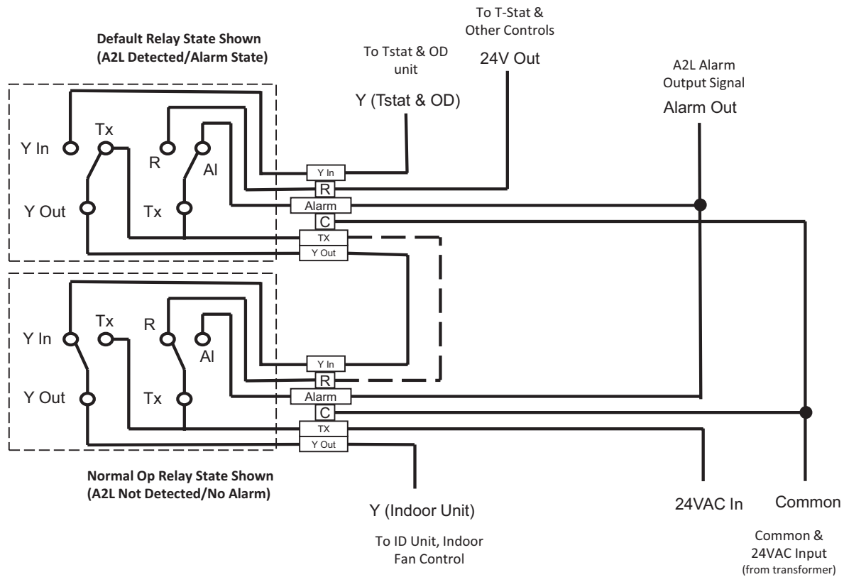
Figure 22. Series Sensor Wiring for systems with 2 or more sensors
