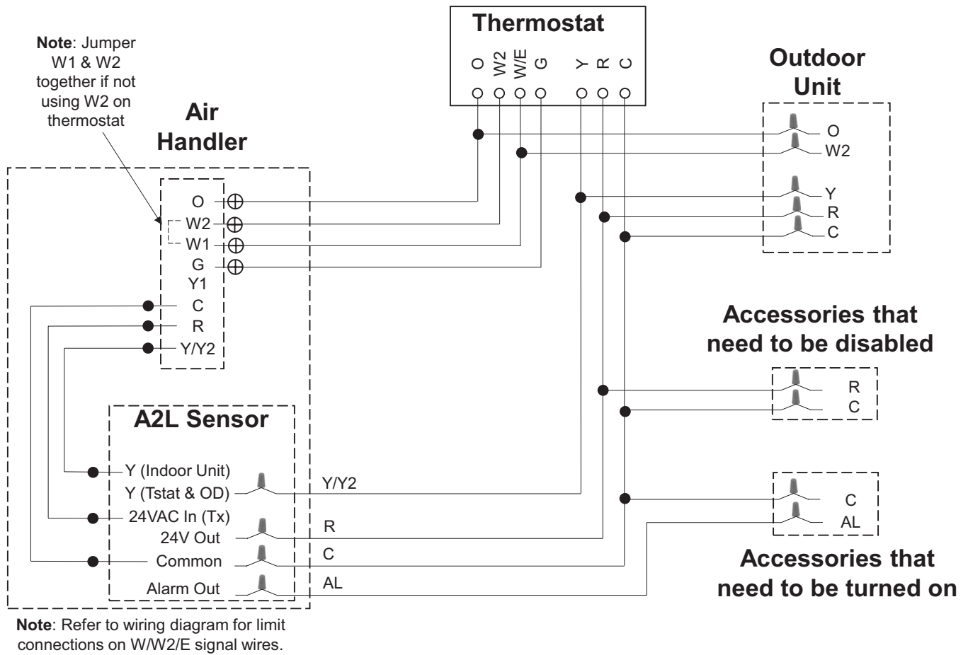
Figure 16. Typical two-stage air handler with single-stage heat pump.
