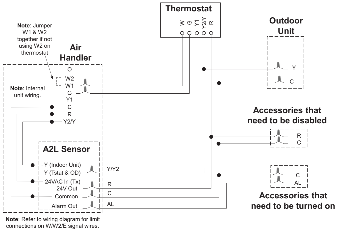
Figure 20. Typical two-stage air handler with single-stage air conditioner.
