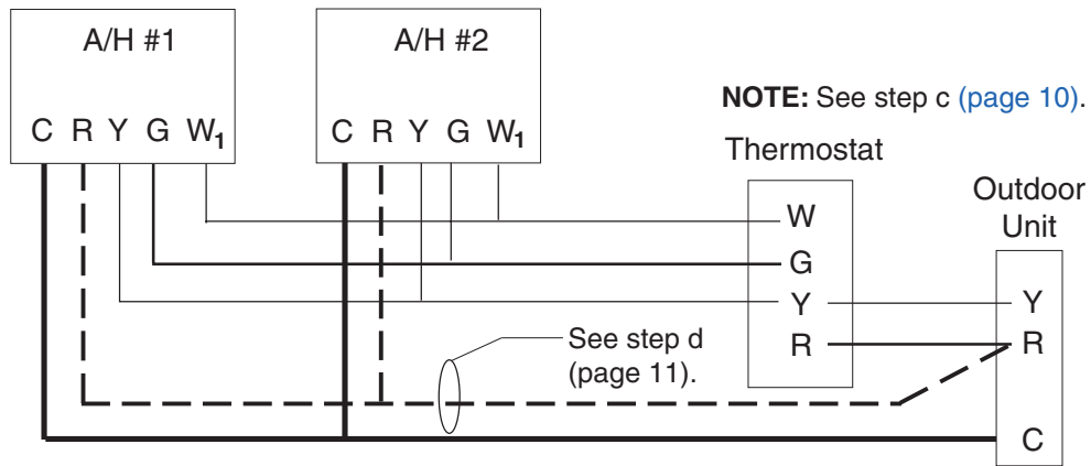
Figure 21. Low Voltage Wiring For Twinning
