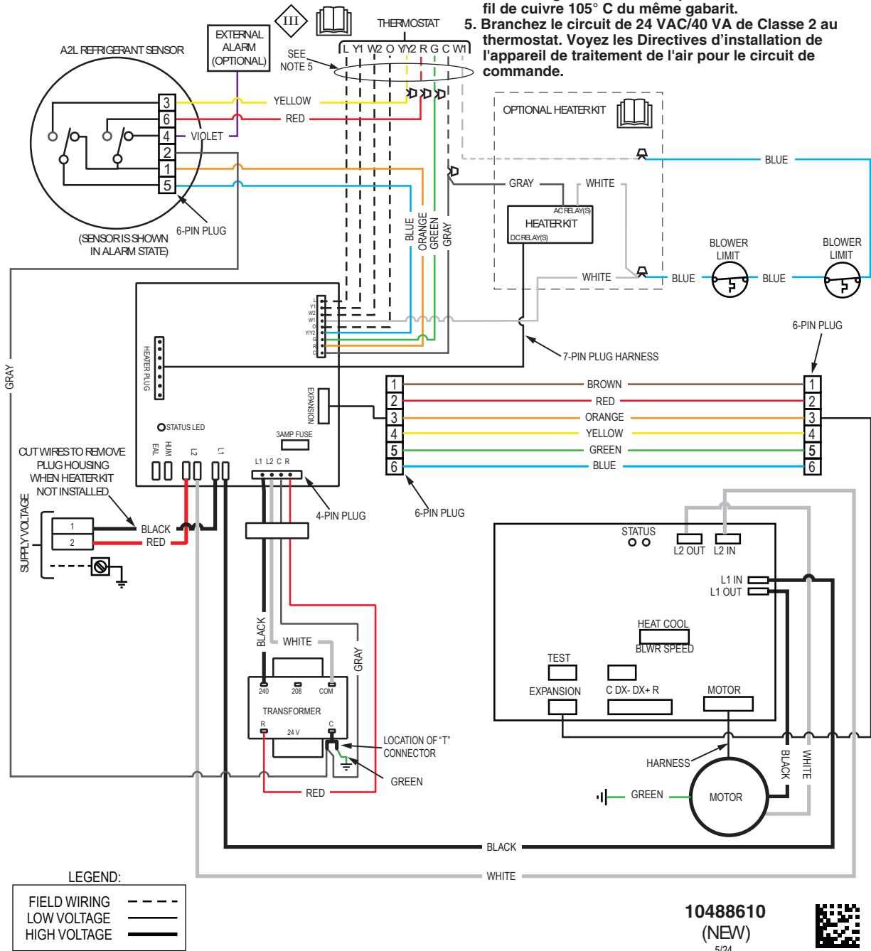
Figure 28 B65VM Wiring Diagram.
