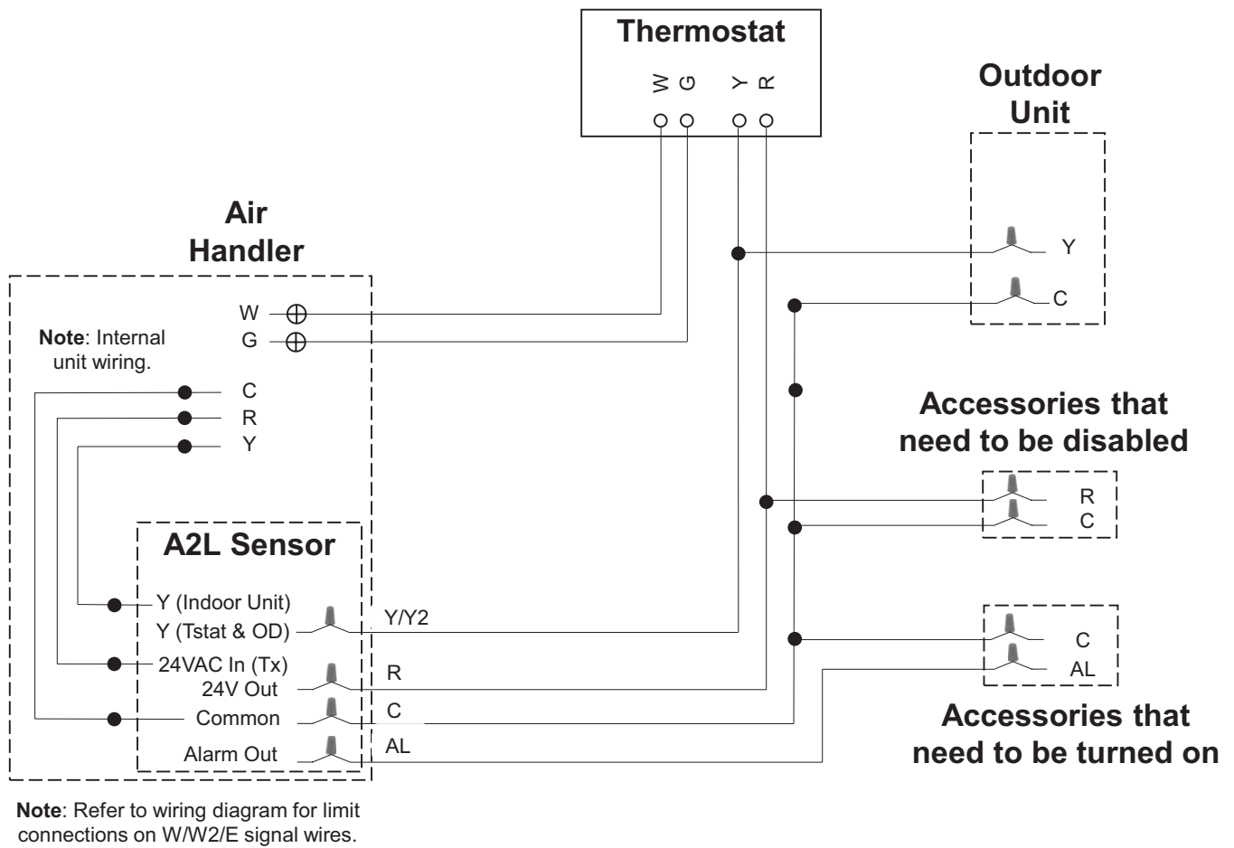
Figure 19. Typical single-stage air handler with single-stage air conditioner.
