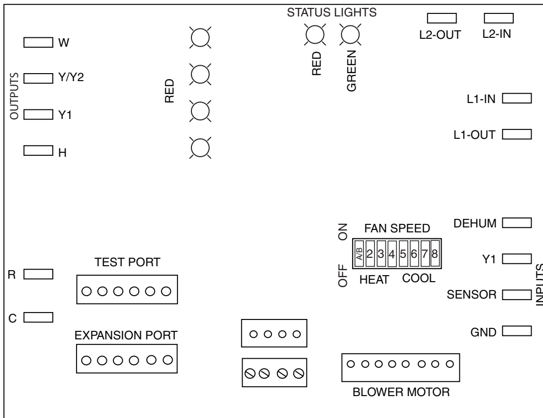
Figure 26. Variable Speed Motor Control Board
