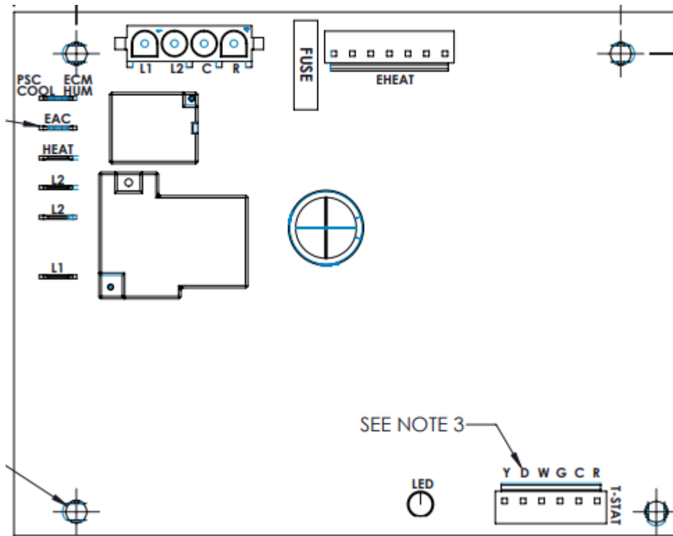
Figure 23. Single Stage Control Board
