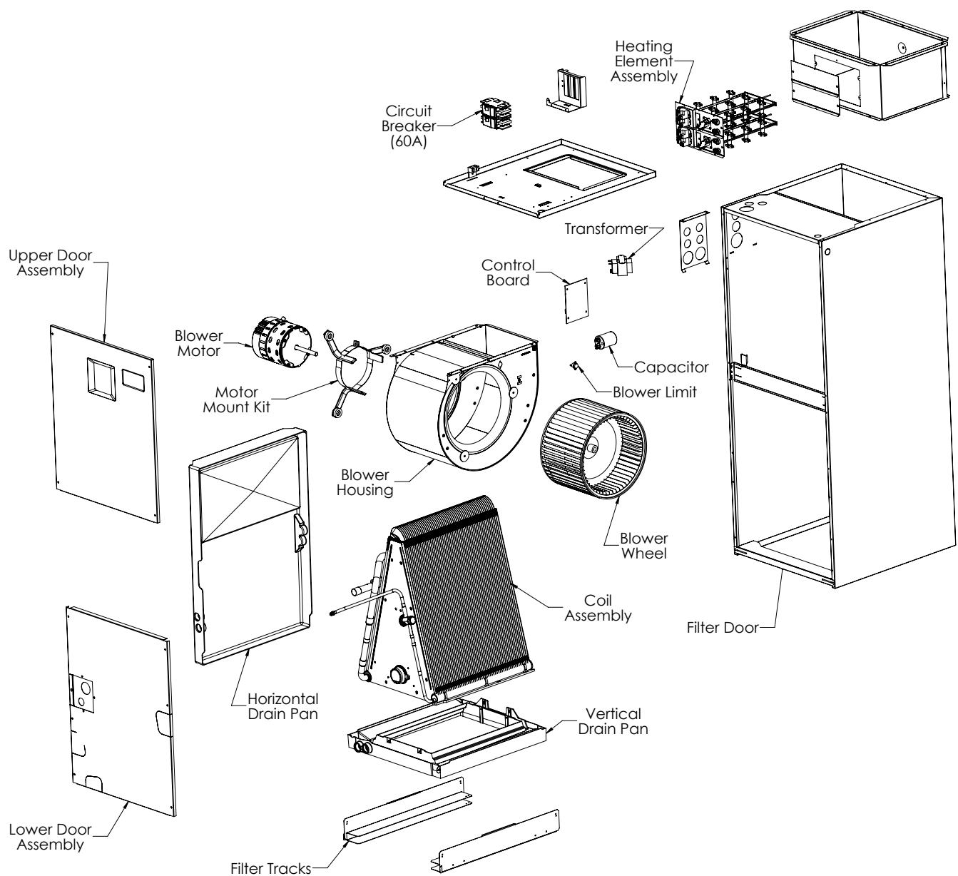
Figure 14. B65BMMX Air Handler Components
