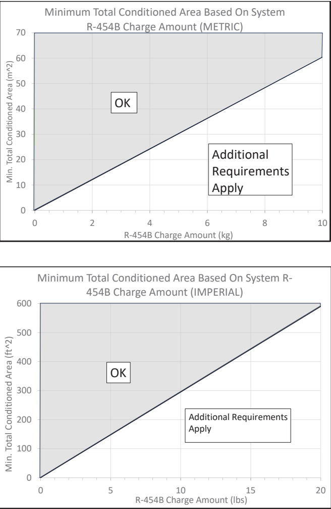
Figure 11. Minimum Total Conditioned Area Based on R-454B System Charge Amount
