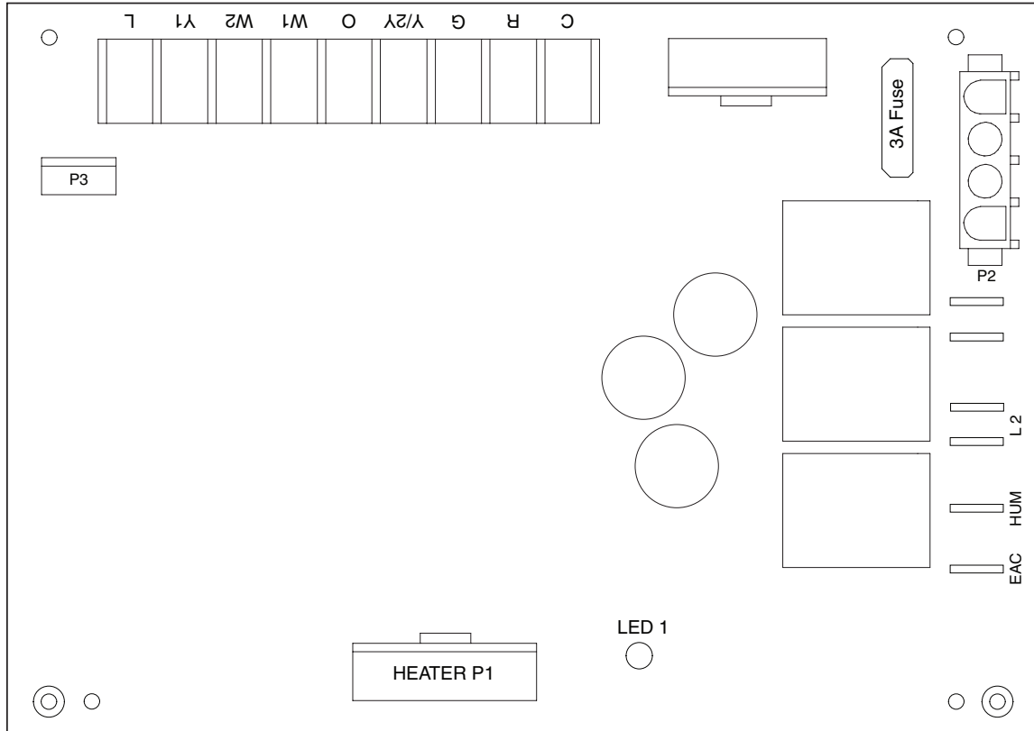
Figure 24. Two - Stage Control Board
