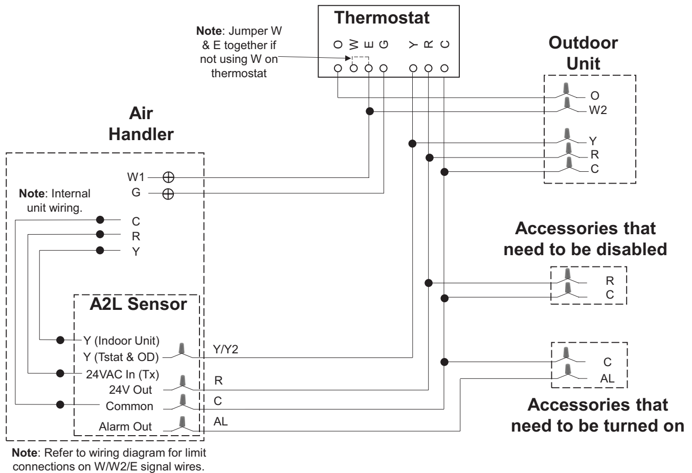
Figure 17. Typical single-stage air handler with single-stage heat pump.
