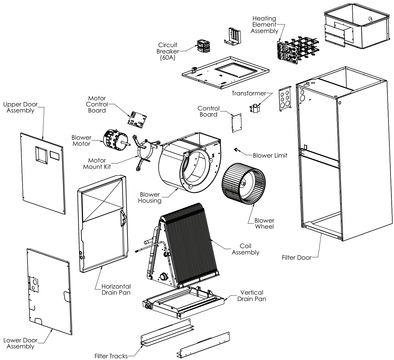
Figure 13. B65(E,V)M Air Handler Components
