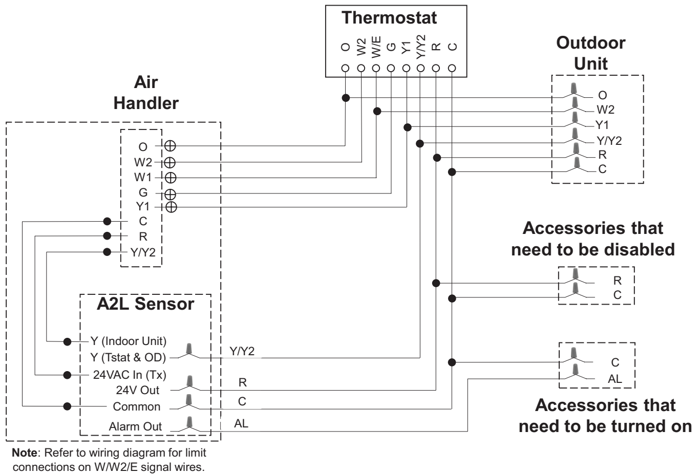
Figure 15. Typical two-stage air handler with two-stage heat pump.
