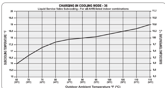
Fig. 15 – Charging in Cooling Mode 25VNA836
