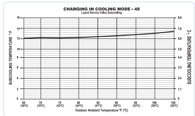
Fig. 24 – Charging in Cooling Mode 24VNA948
