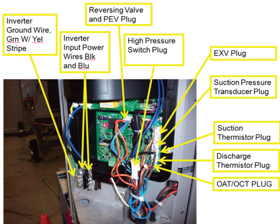
Fig. 41 – Wire Harness Connections (Unit sizes 24A, 25, 36, 37, 48, 49 and 60)
