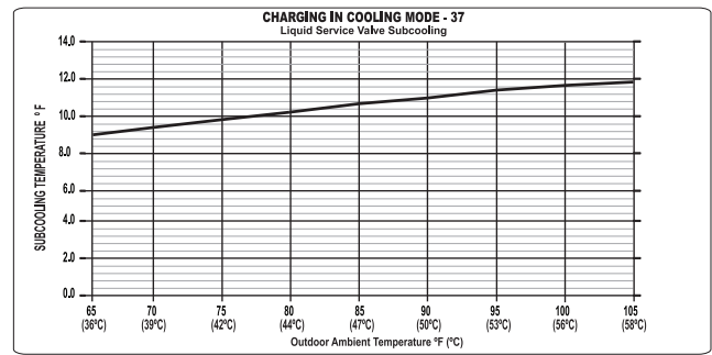
Fig. 16 – Charging in Cooling Mode 25VNA837
