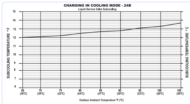
Fig. 21 – Charging in Cooling Mode 24VNA924B
