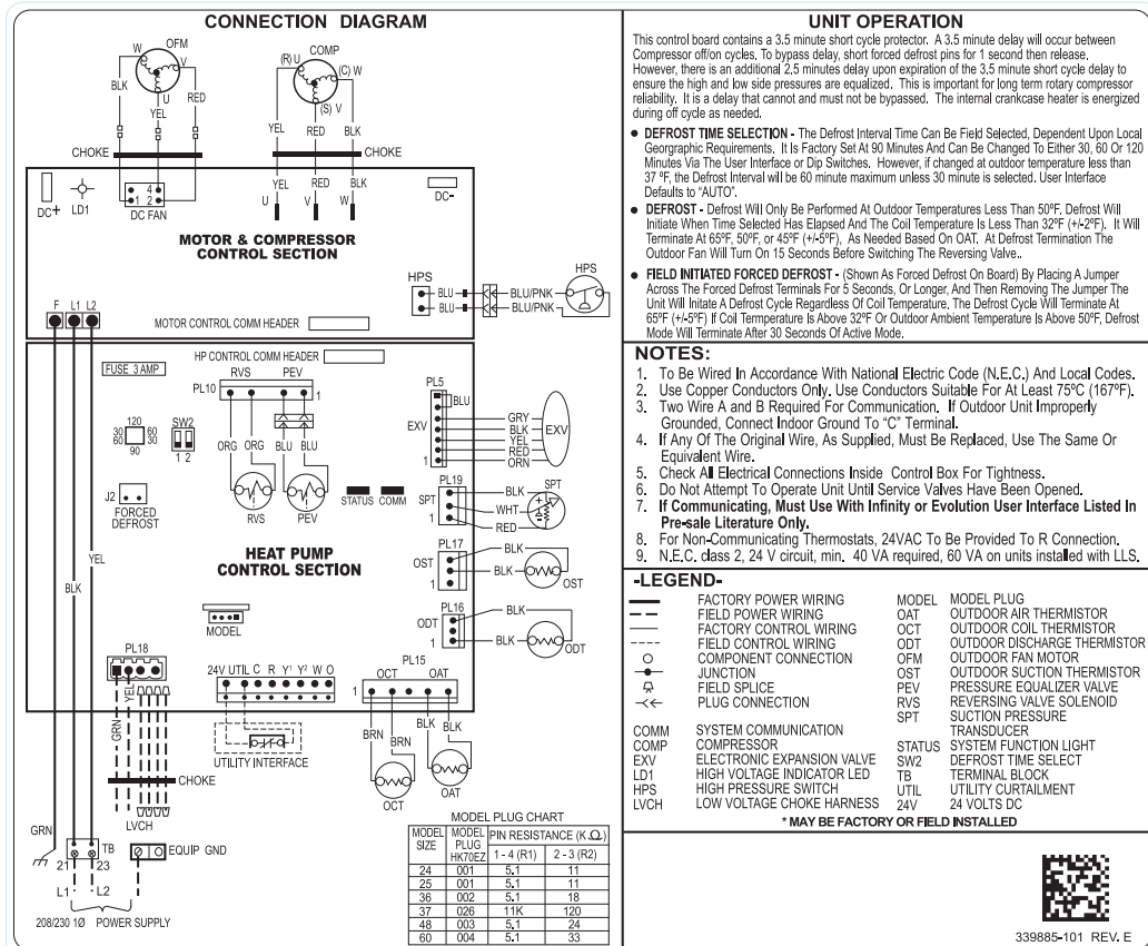
Fig. 46 – 25VNA8 WIRING DIAGRAM - Sizes 24A, 25, 30, 36, 37, 48, and 60
