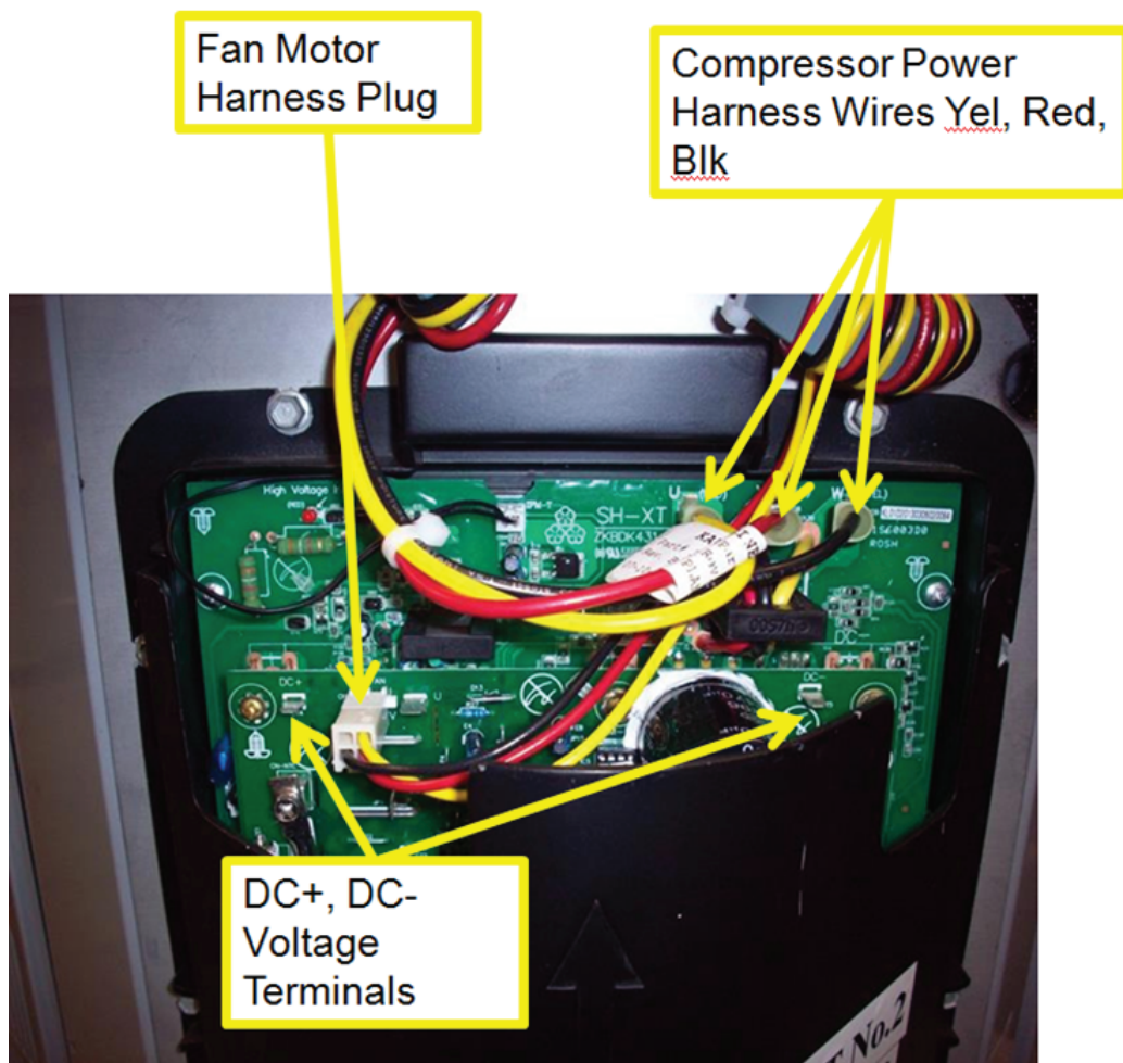
Fig. 39 – Compressor and Fan Harness (Unit sizes 24A, 25, 36, 37, 48, 49 and 60)
