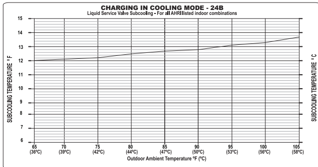
Fig. 14 – Charging in Cooling Mode 25VNA824B
