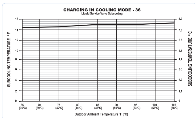
Fig. 22 – Charging in Cooling Mode 24VNA936
