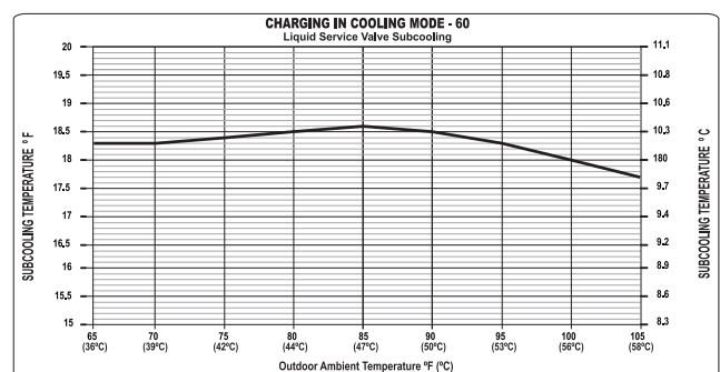
Fig. 18 – Charging in Cooling Mode 25VNA860
