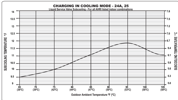
Fig. 13 – Charging in Cooling Mode 25VNA824A/25
