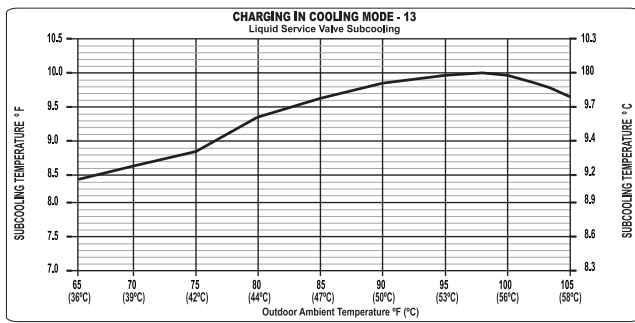
Fig. 12 – Charging in Cooling Mode 25VNA813
