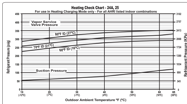
Fig. 28 – Heating Pressure Check Chart 25VNA824A, 25
