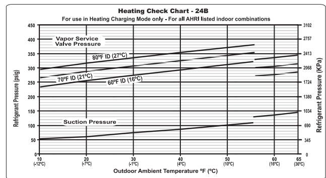
Fig. 29 – Heating Pressure Check Chart 25VNA824B
