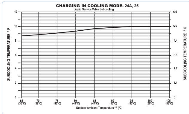
Fig. 20 – Charging in Cooling Mode 24VNA924A/25
