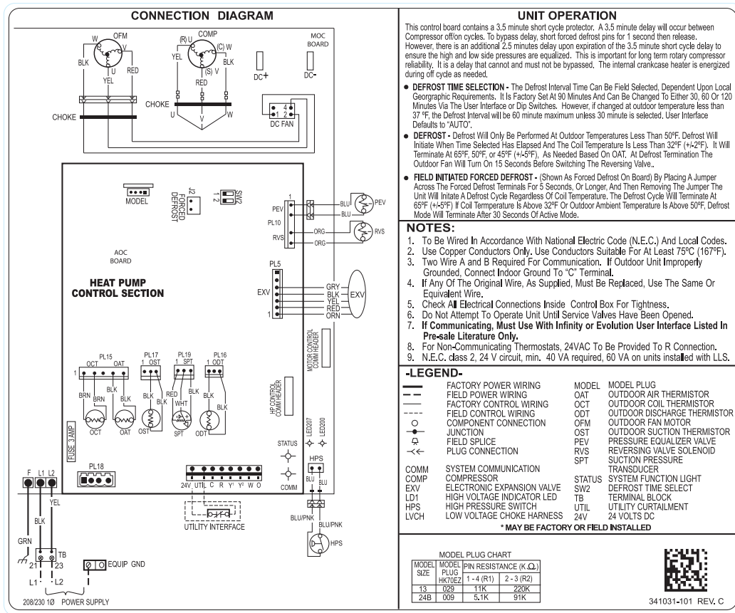
Fig. 45 – 25VNA8 WIRING DIAGRAM - Sizes 13 and 24B
