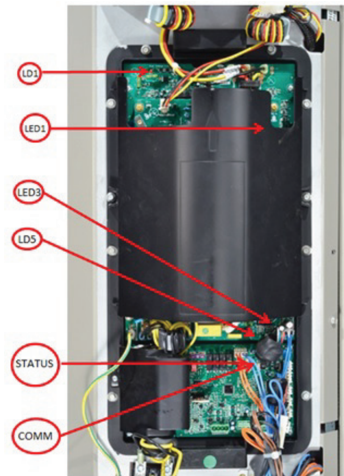
MOC LED Description (Sizes 24A, 25, 36, 37, 48, 49 AND 60)
