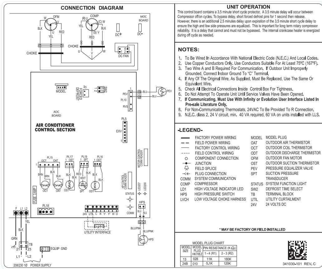
Fig. 43 – 24VNA9 WIRING DIAGRAM - Sizes 13 and 24B
