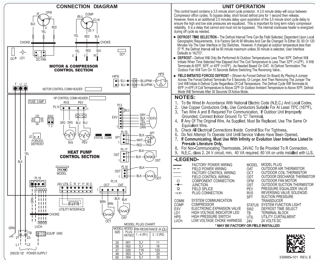
Fig. 46 – 25VNA8 WIRING DIAGRAM - Sizes 25, 36, 37, 48, and 60
