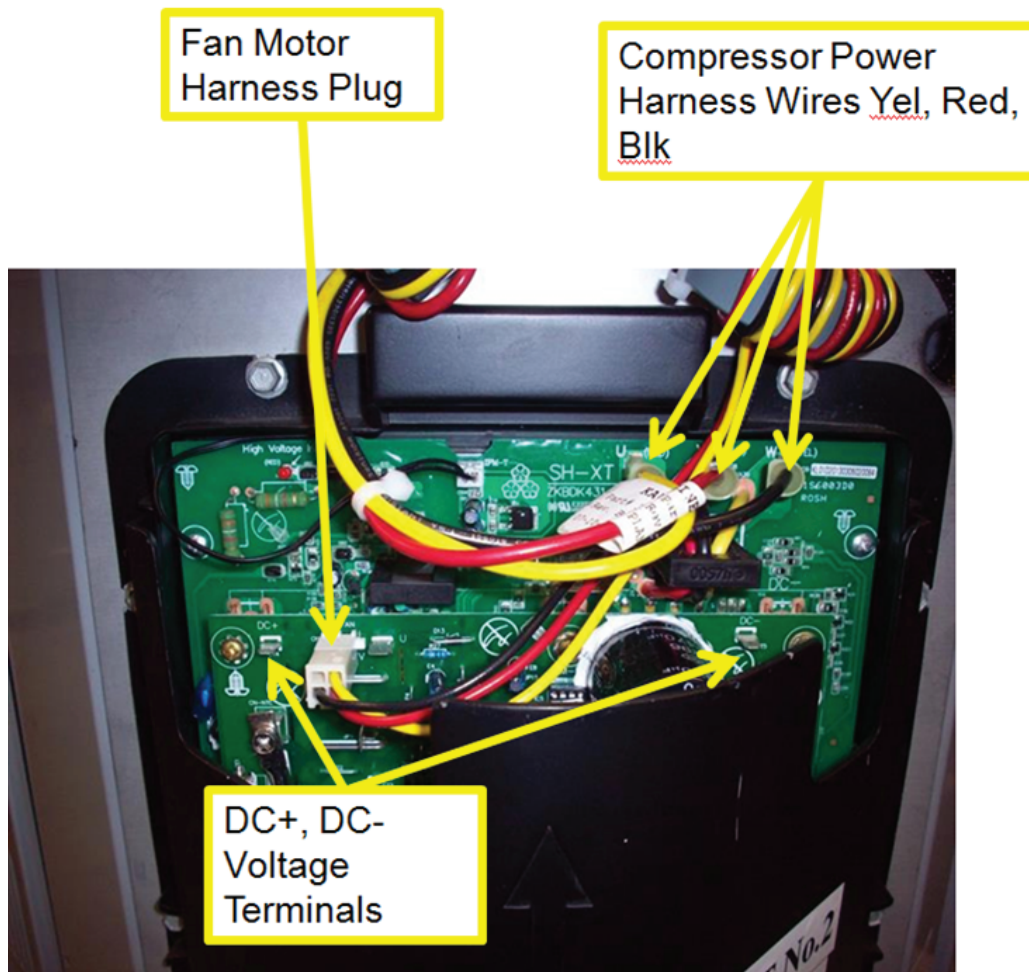
Fig. 40 – Compressor and Fan Harness (Unit sizes 25, 36, 37, 48, 49 and 60)
