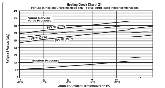
Fig. 28 – Heating Pressure Check Chart 25VNA824
