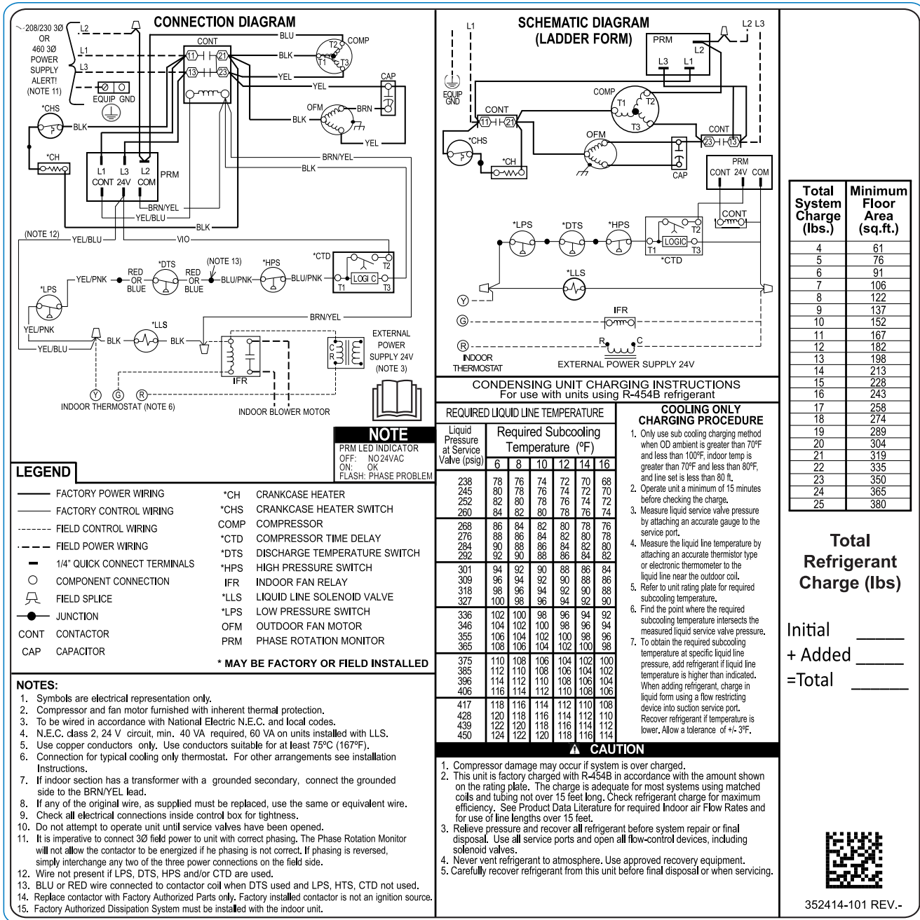
Fig. 2 – Sizes 36 - 60 208-230-3 & 460-3
