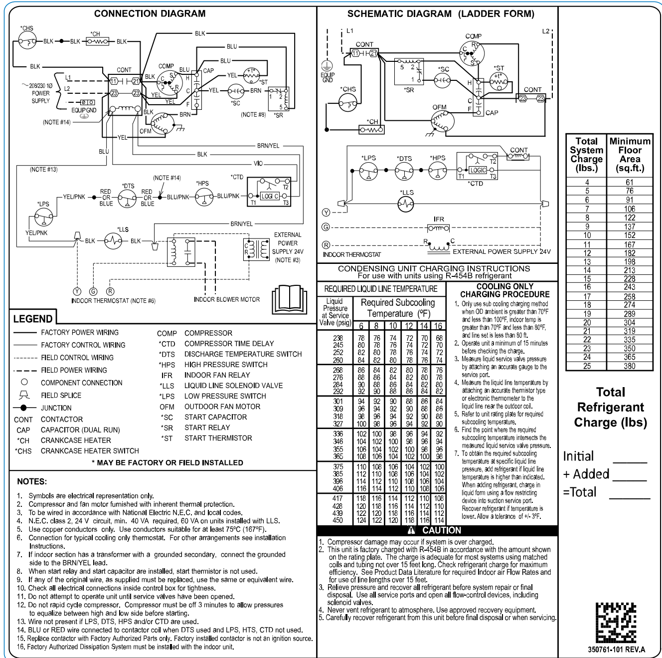
Fig. 1 – Sizes 18 - 60 208-230-1
