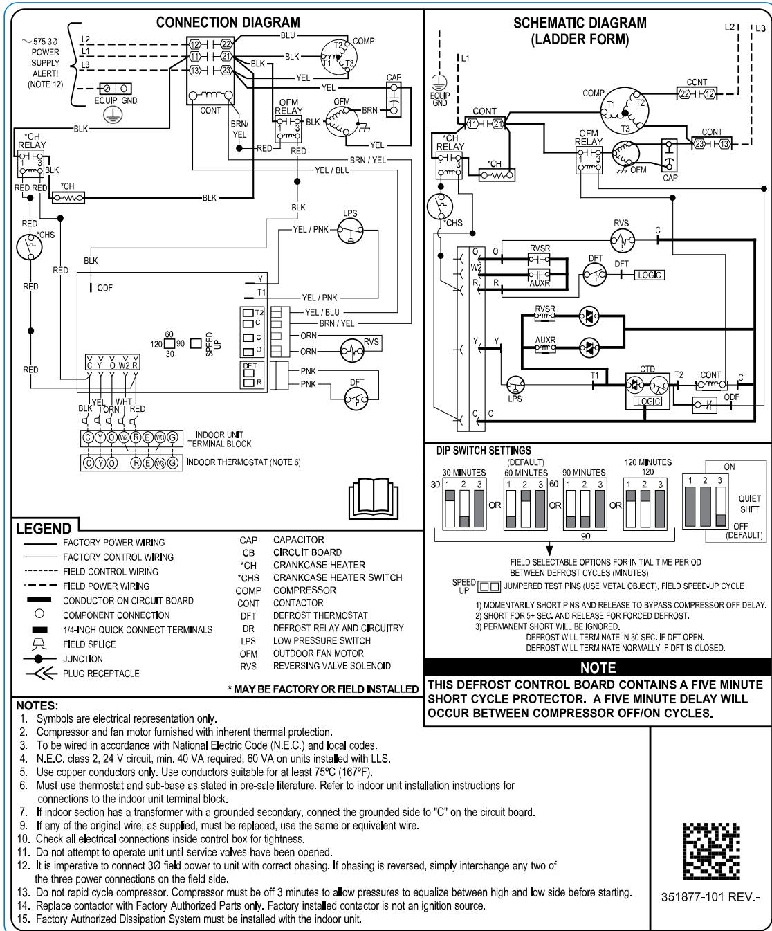
Fig. 4 – 575-3-60 Sizes (3, 4 and 5 Tons)
