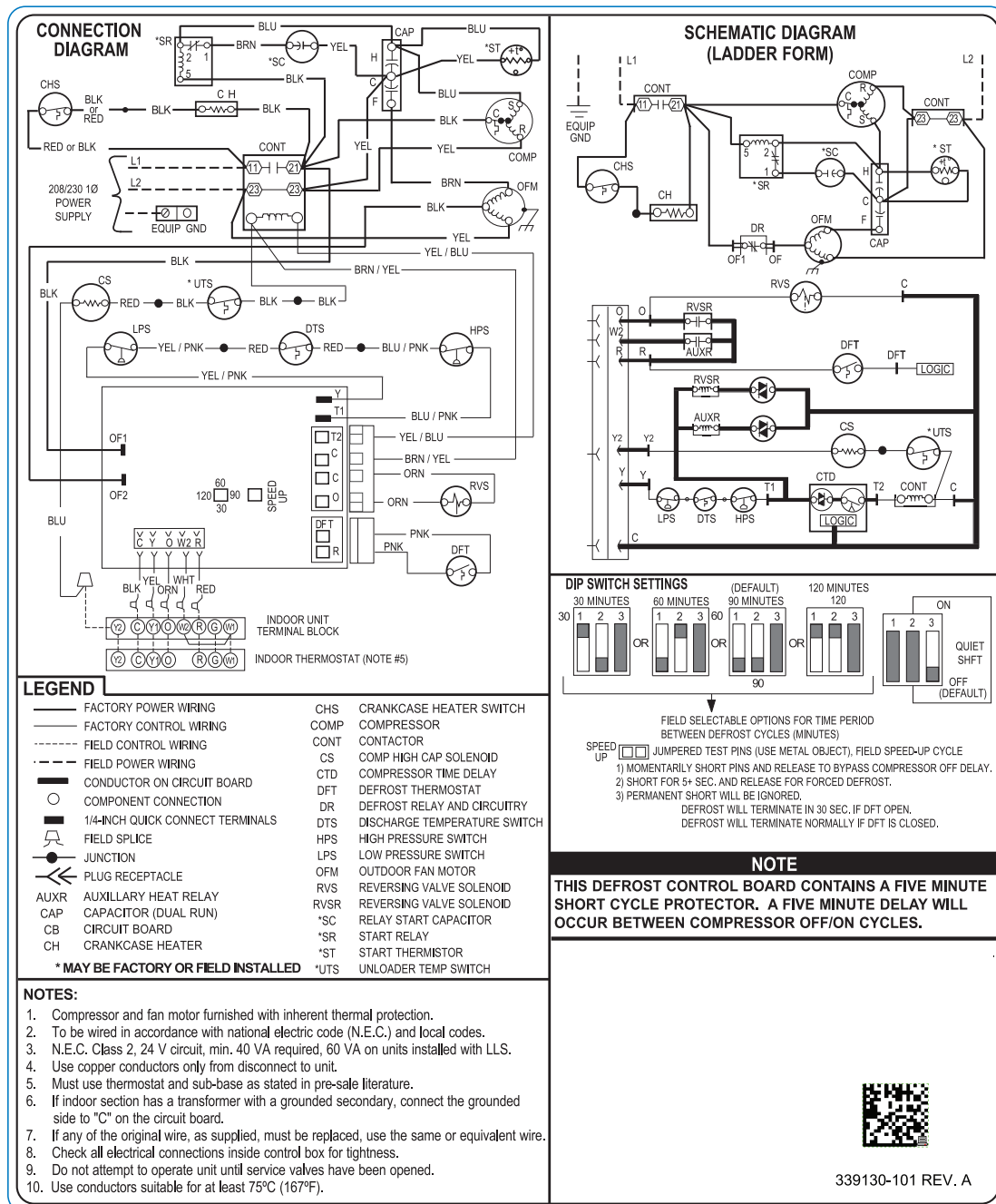
Fig. 1 – PH16NA 2 - 5 Tons
