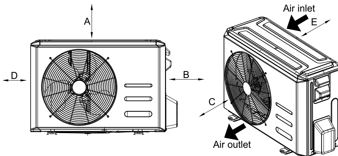
Fig. 3 – Outdoor Unit Clearances
