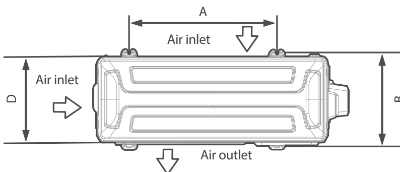
Fig. 2 – System Sizes and Mounting Dimensions (all Models)
