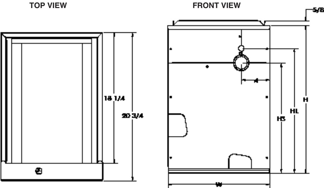
Figure 1. C75 Coil Dimensions (with fixed orifice)
