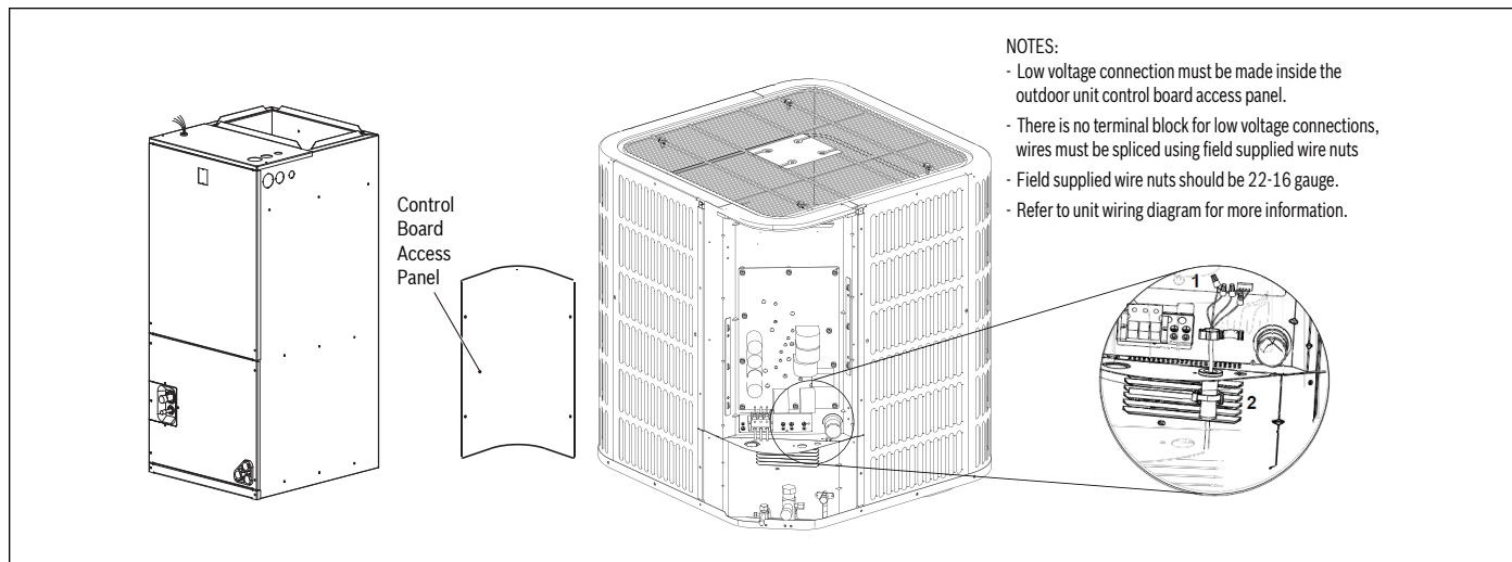
Figure 30 Low Voltage Unit Connections
