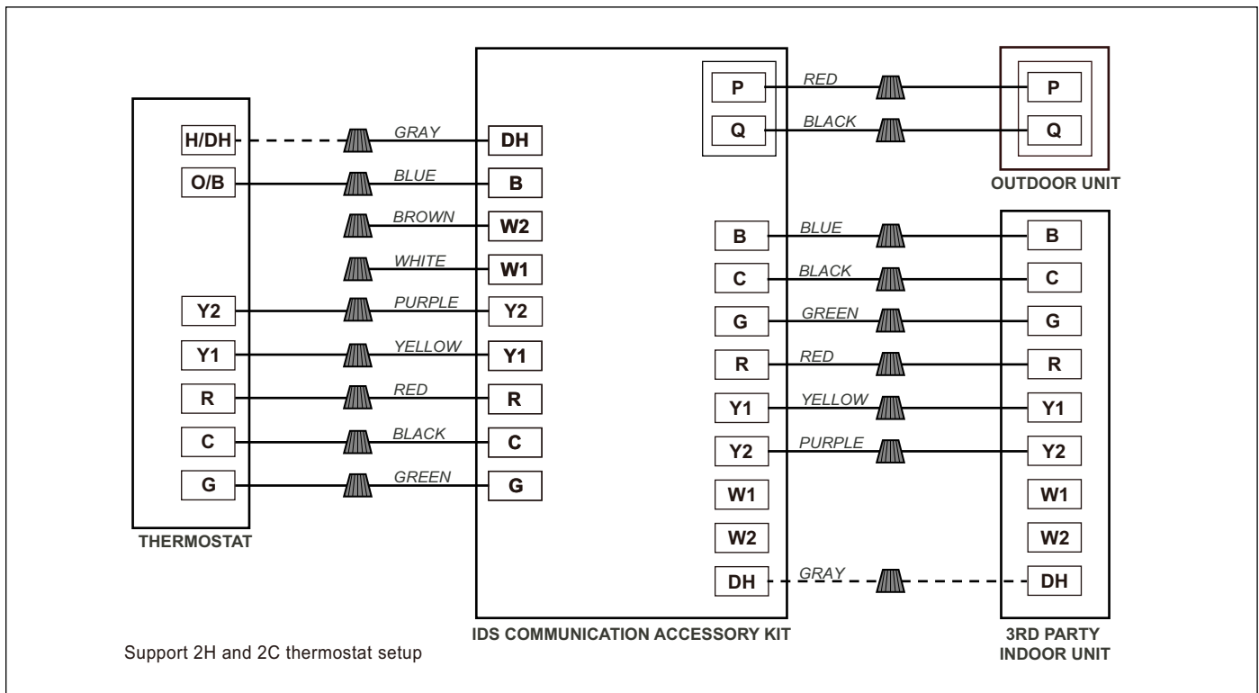
Figure 42 Control wiring for IDS Communication Accessory Kit
