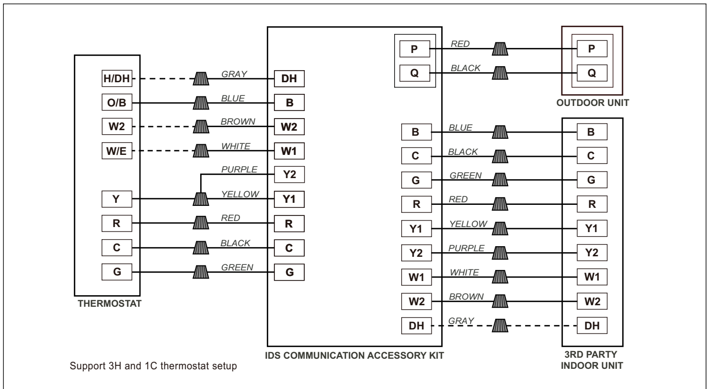
Figure 41 Control wiring for IDS Communication Accessory Kit
