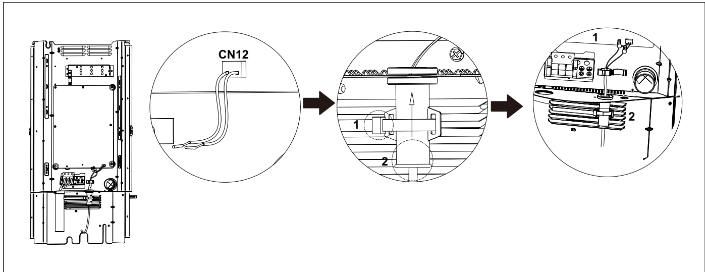
Figure 32 Wires connections diagram
