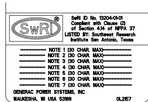
Figure 3-3. Southwest Research Institute Marking
