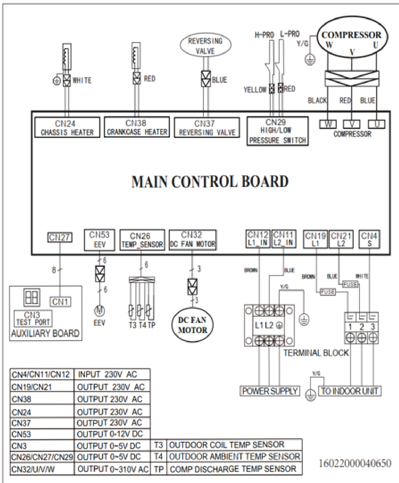
Fig. 7 —36K – 208/230V Wiring Diagram
