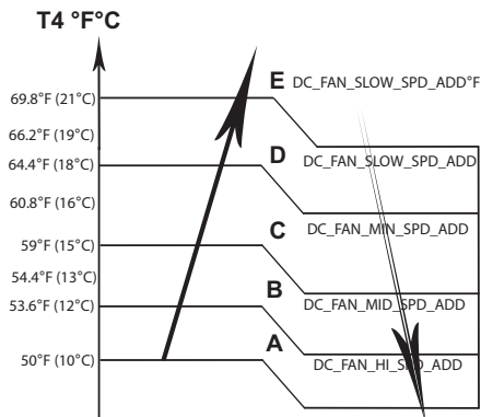
Fig. 21 —Outdoor Fan Running Rules
