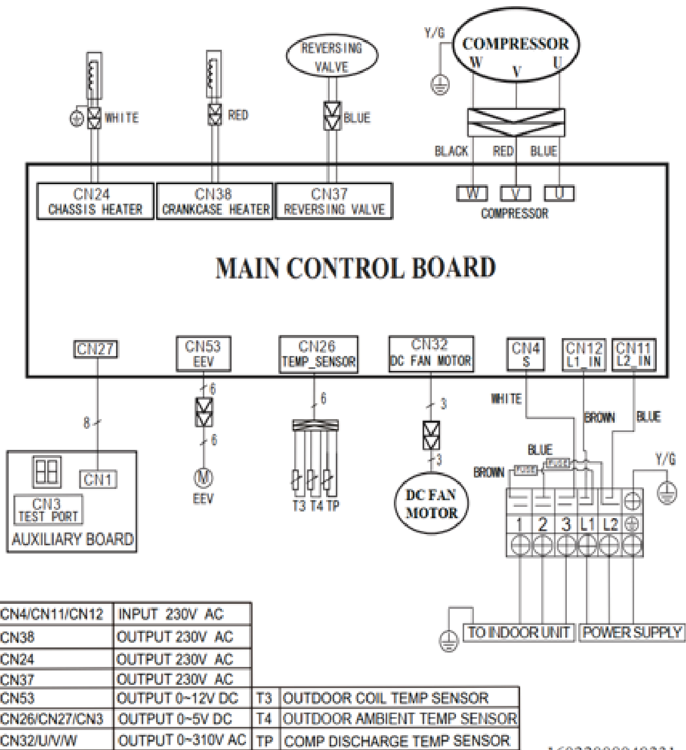
Fig. 6 —30K – 208/230V Wiring Diagram
