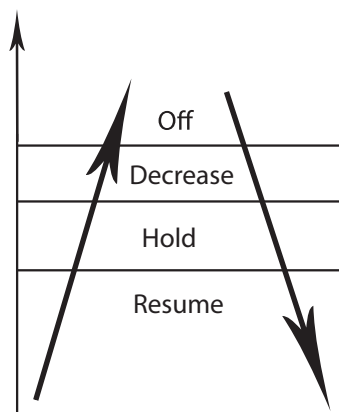
Fig. 17 —Evaporator Coil Temperature Protection
