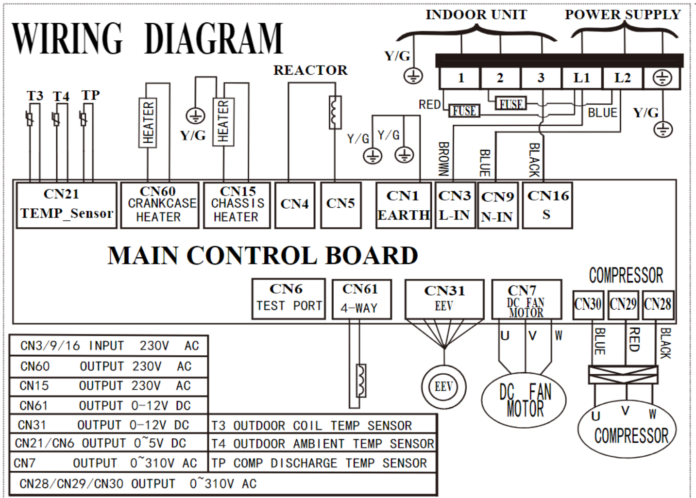
Fig. 4 —Wiring Diagram (Sizes 6K - 12K)
