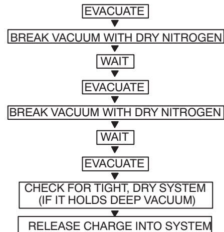
Fig. 11 —Triple Evacuation Method
