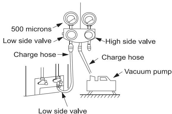
Fig. 9 —Manifold
