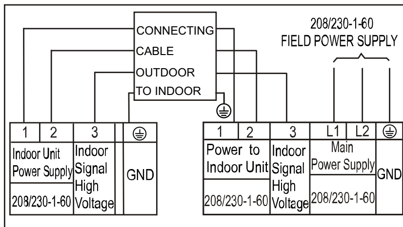
Fig. 3 — Connection Diagram Sizes 6K - 18K
