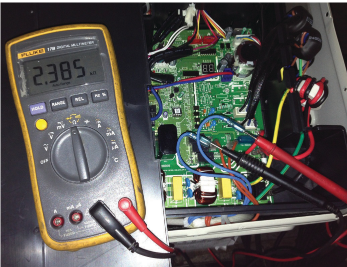
Fig. 32 —Use a Digital Tester to Measure Resistance
