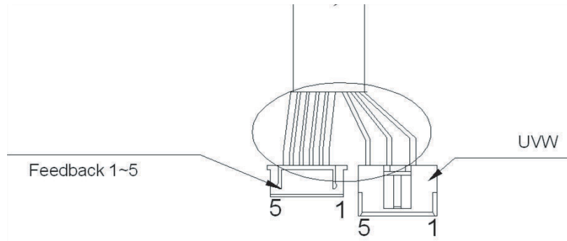
Fig. 26 —Outdoor DC Fan Motor (DC motor that controls the chip on the PCB)
