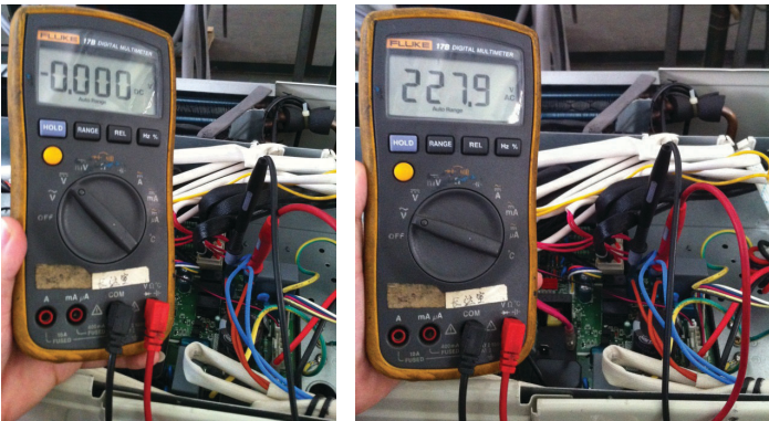
Fig. 31 —Measure the Voltage
