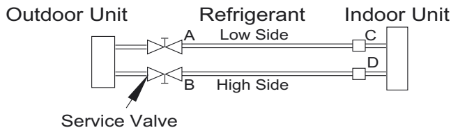
Fig. 8 —Service Valve
