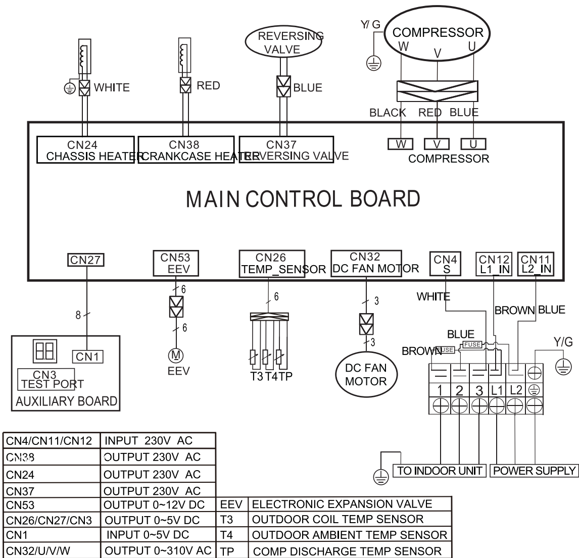
Fig. 5 —Wiring Diagram (Size 18K)
