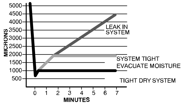
Fig. 10 —Deep Vacuum Graph
