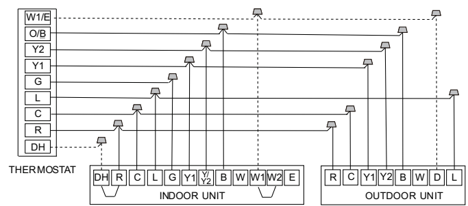
Fig. 10 —Wiring for 3H and 2C Thermostat
