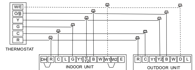
Fig. 12 — Wiring for 2H and 1C Thermostat
