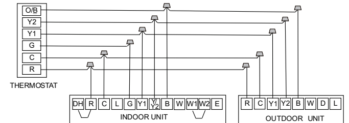
Fig. 11 —Wiring for 2H and 2C Thermostat
