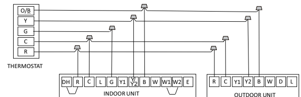
Fig. 13 —Wiring for 1H and 1C Thermostat
