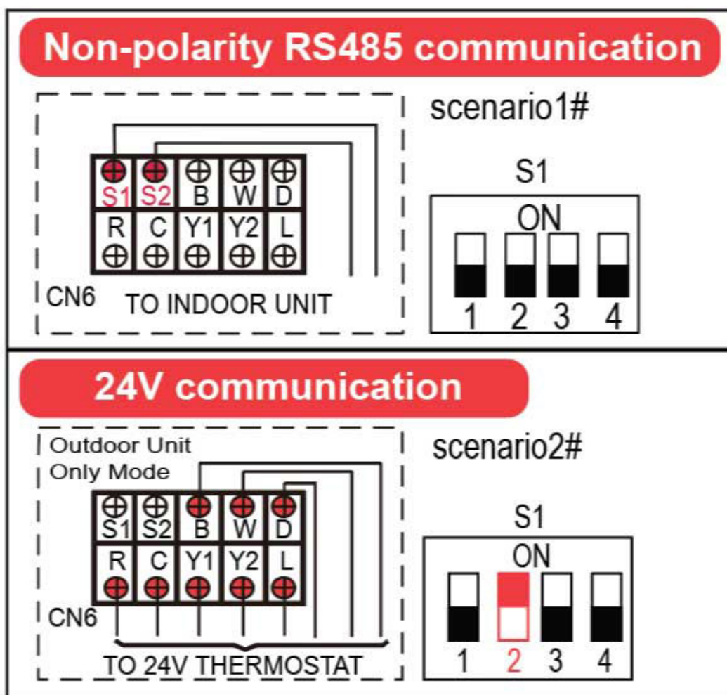
Fig. 6 —Connection Diagrams
