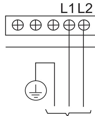
Fig. 2 — Match Fork Terminal to Terminal Labels
