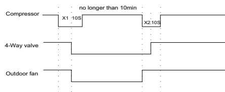
Fig. 14 — Defrost Action
