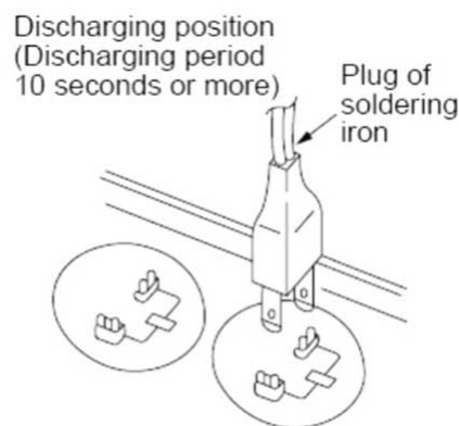
Fig. 17 — Discharging Position
