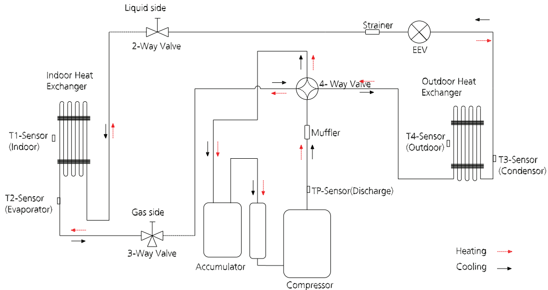
Fig. 3 — Refrigerant Cycle Diagram (Sizes 6K-9K)
