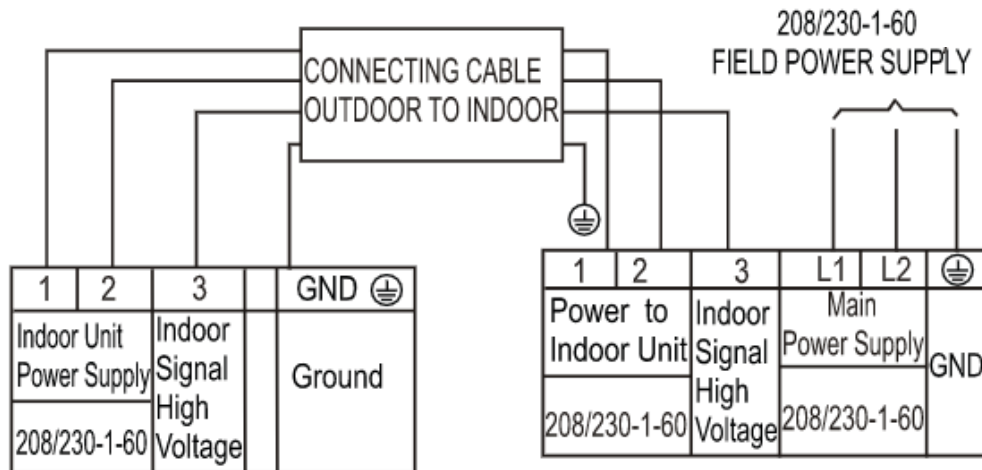
Fig. 1 — Connection Diagram - Sizes 06K-18K
