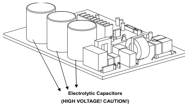
Fig. 16 — Capacitors
