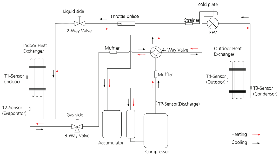
Fig. 4 — Refrigerant Cycle Diagram (Sizes 12K-18K)
