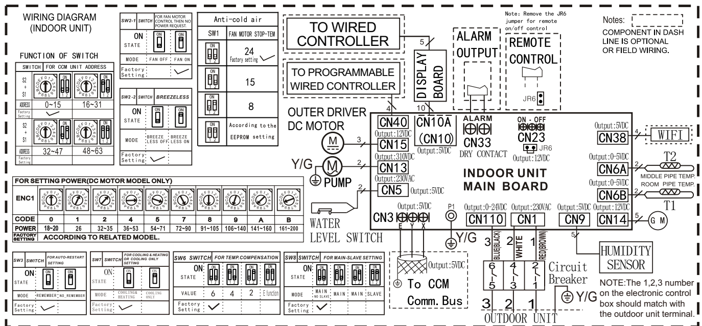
Fig. 2 — Wiring Diagram - Sizes 06K-18K
