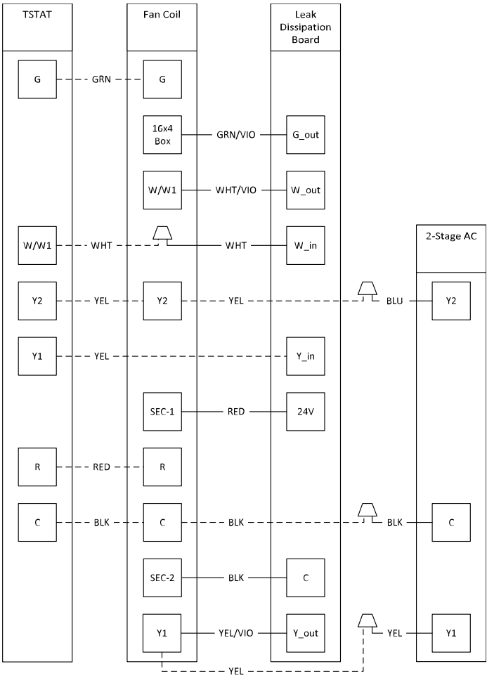
Fig. 8 – Thermostat with Fan Coil, Leak Dissipation Board and 2-Stage AC
