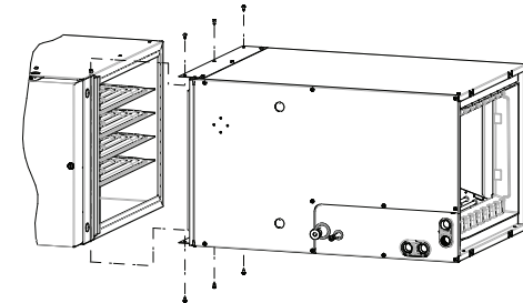
Fig. 5 - Horizontal Right Installation
