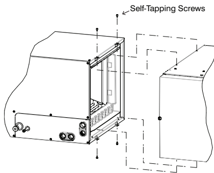
Fig. 7 - Horizontal Left Installation
