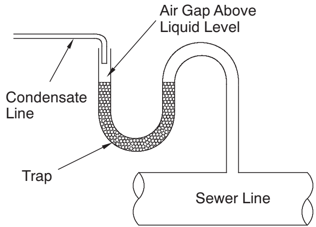
Fig. 9 - Condensate Drain to Waste Line
