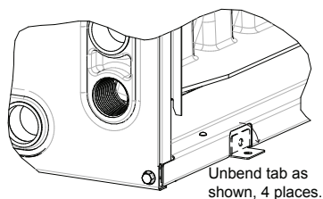
Fig. 6 - Horizontal Left Installation
