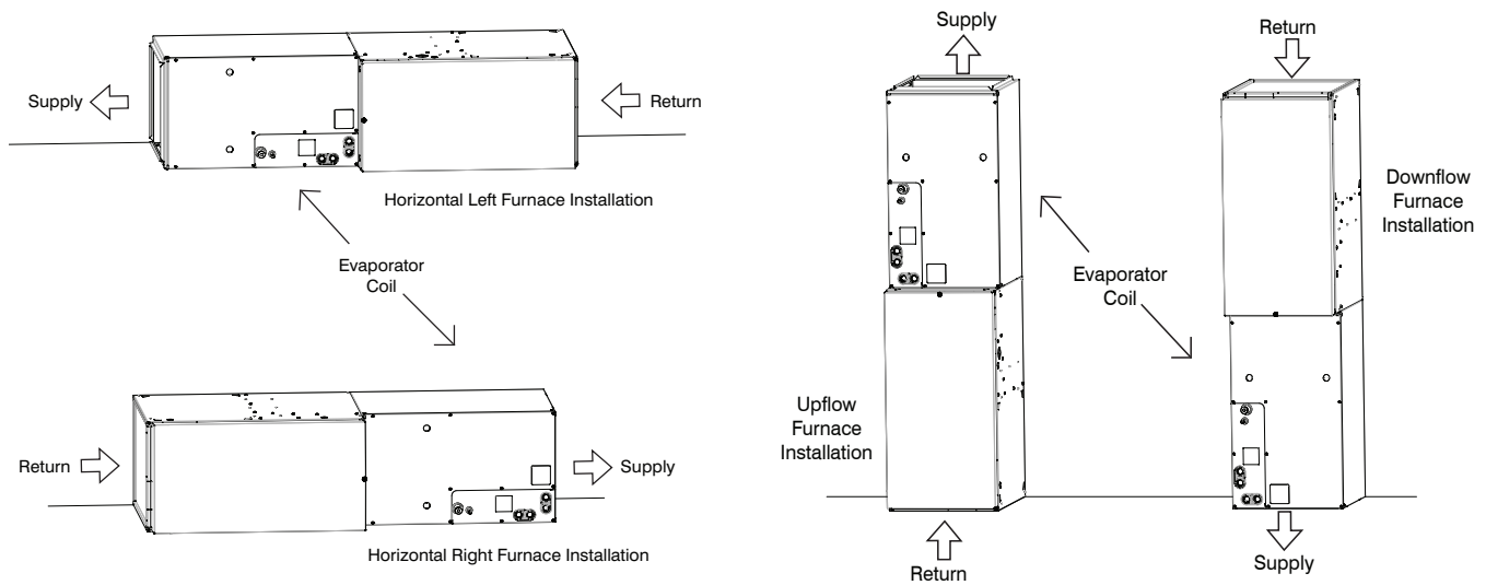
A13059 Fig. 1 - Typical Installation Multipoise Cased Coils
