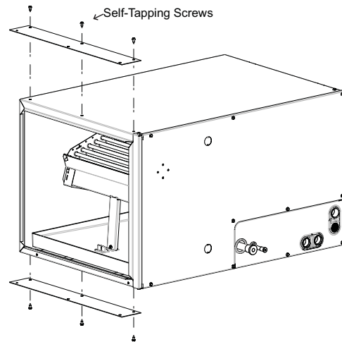
Fig. 4 - Horizontal Right Installation
