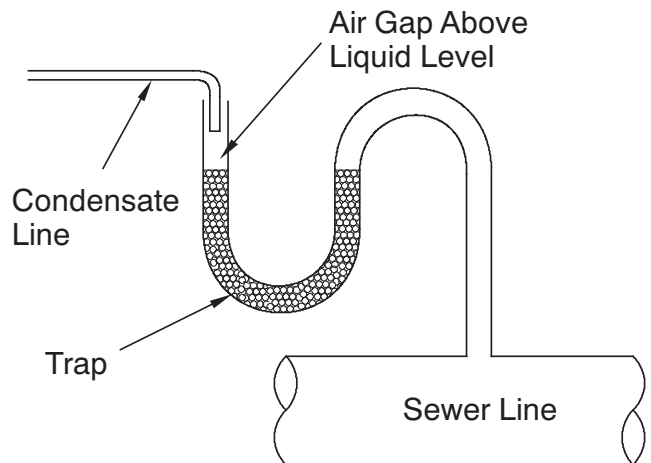
Fig. 9 - Condensate Drain to Waste Line
