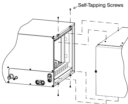
Fig. 7 - Horizontal Left Installation
