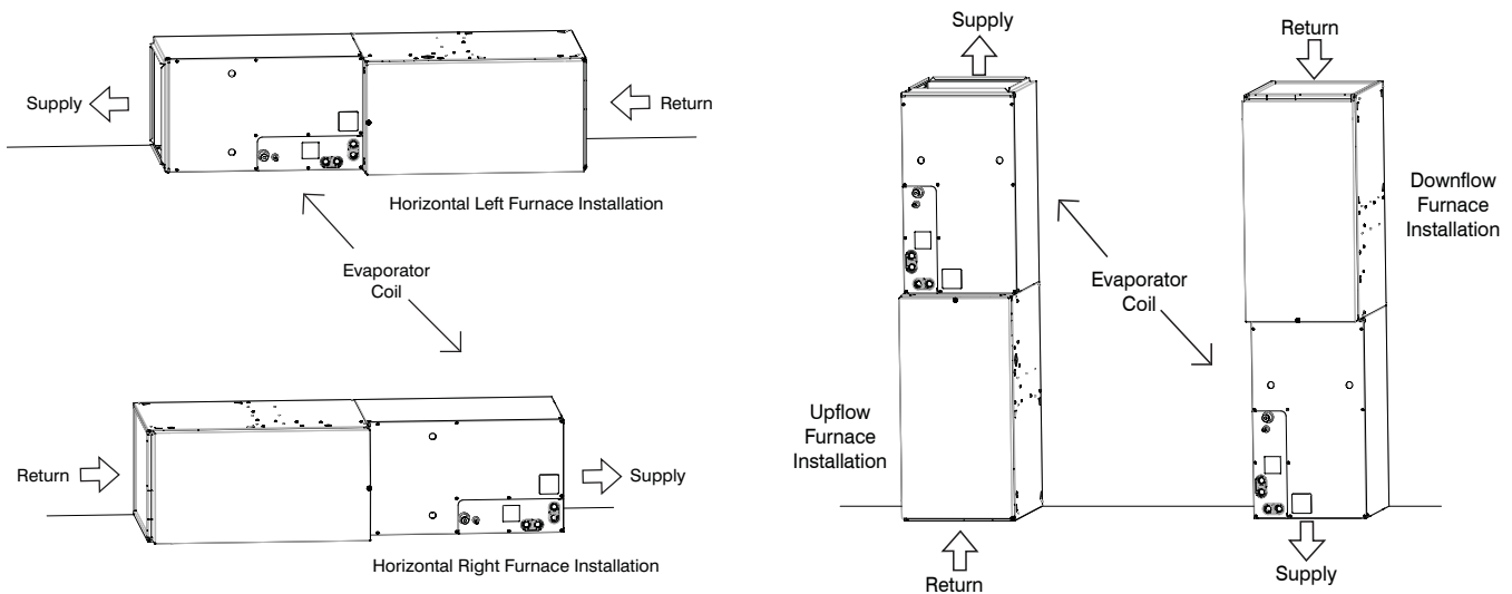
Fig. 1 - Typical Installation Multipoise Cased Coils
