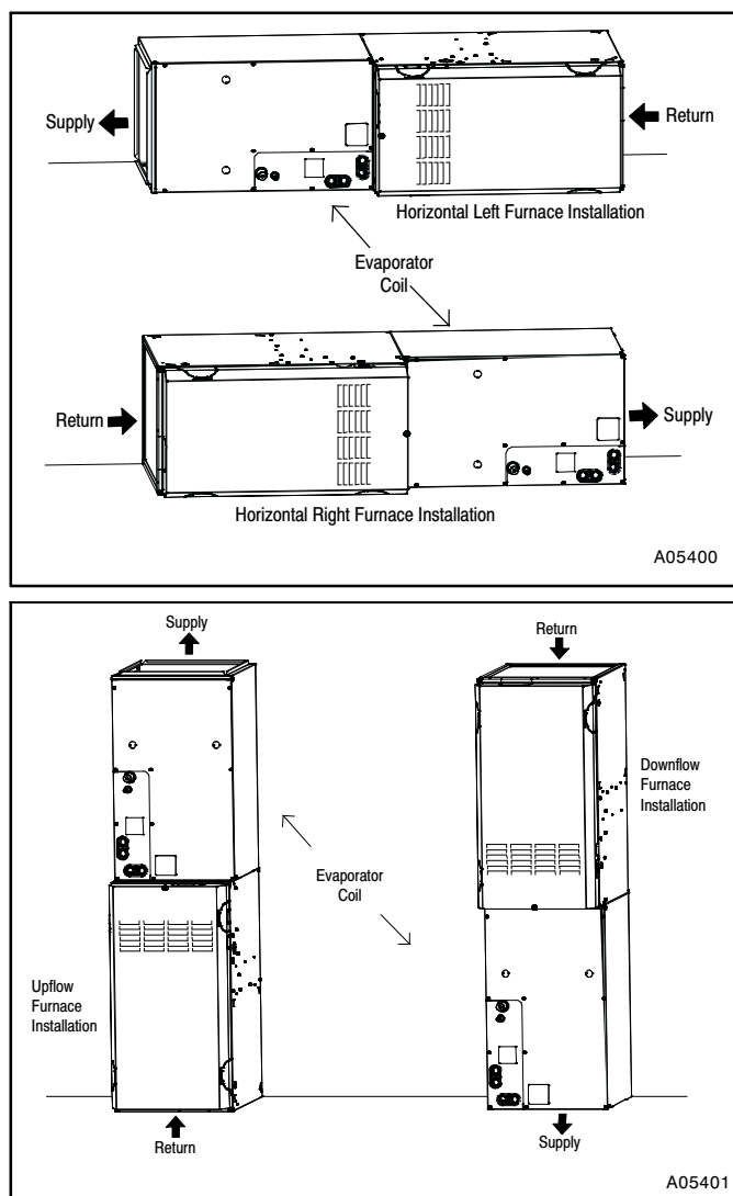
Figure 1 – Typical Coil Installation on Furnace
