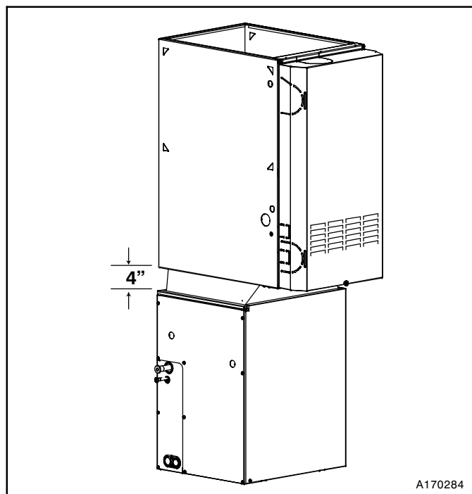
Figure 3 – Downflow Installation with Coil Rotated 90°
