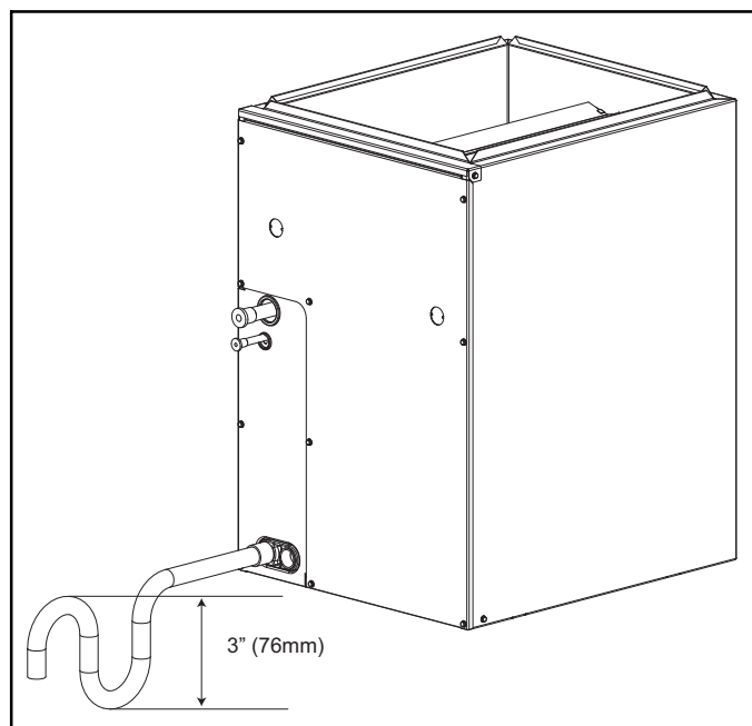
Figure 9 – Condensate Trap
