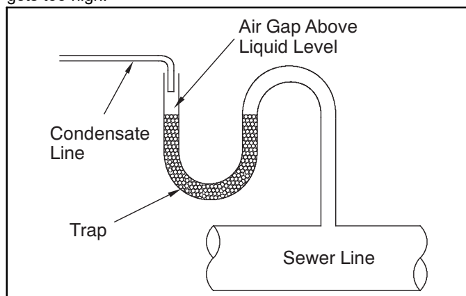
Figure 10 – Condensate Drain to Waste Line
