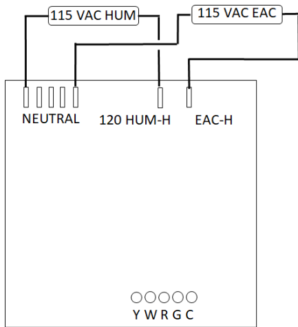
Accessory Wiring
