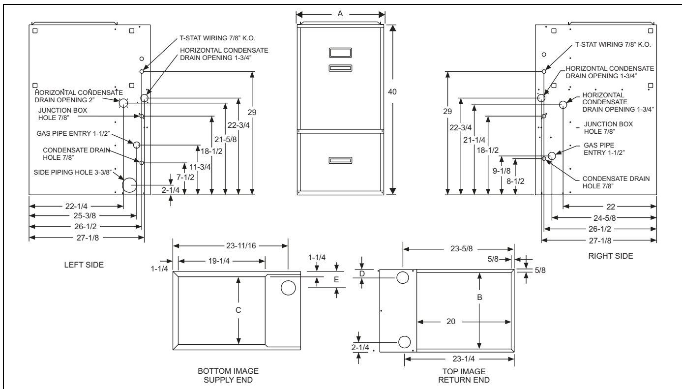
FIGURE 3: Dimensions
