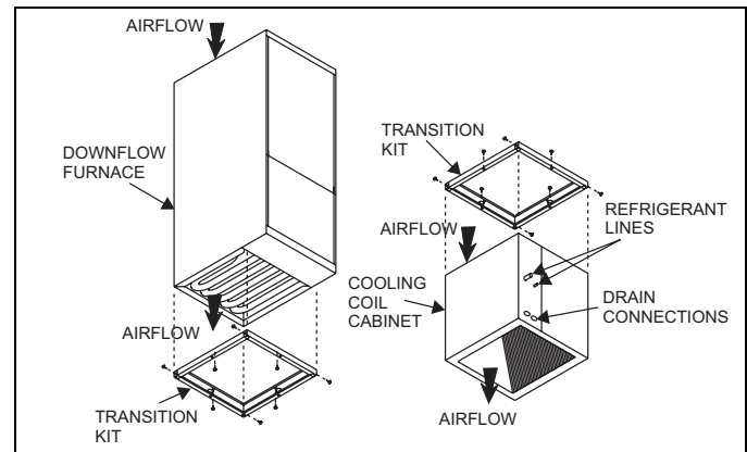
FIGURE 2: Transition Kit Assembly
