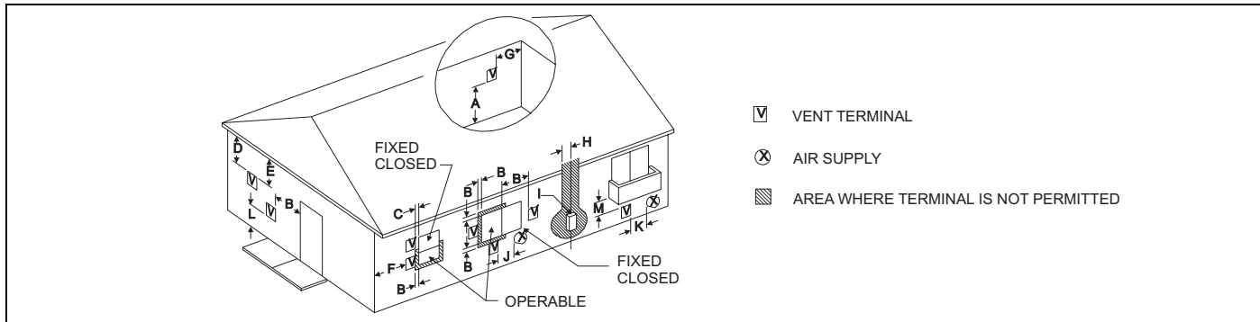
FIGURE 16: Home Layout
