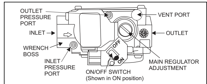
FIGURE 38: Gas Valve
