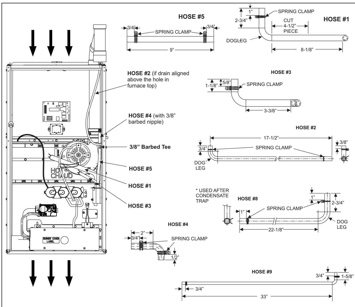
FIGURE 30: Downflow Condensate Drain Hose Configuration
