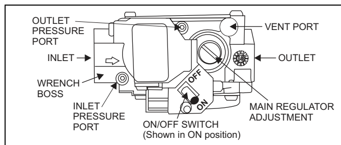
FIGURE 7: Gas Valve
