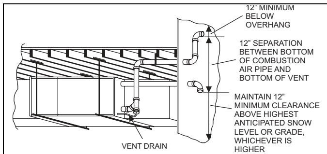
FIGURE 22: Crawl Space Termination Configuration - 2 Pipe
