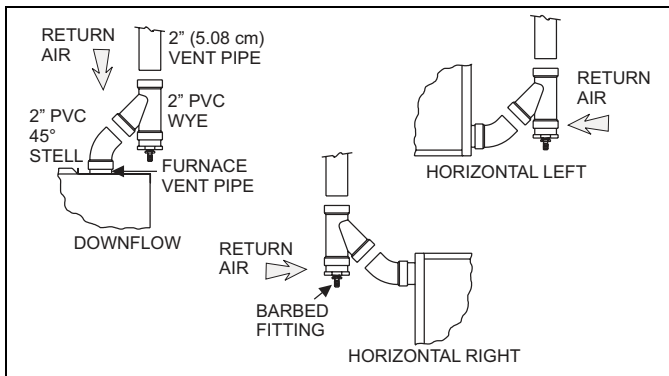
FIGURE 17: Downflow/Horizontal Vent Assembly
