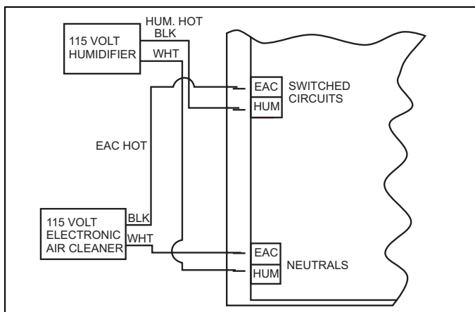
FIGURE 12: Accessory Connections
