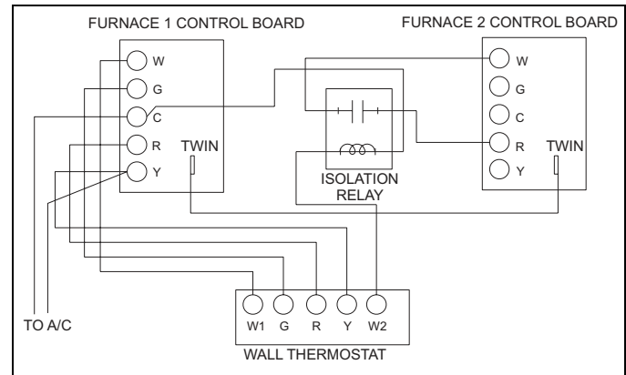
FIGURE 15: Two-Stage Twinning Wiring Diagram
