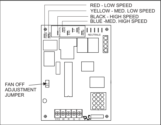
FIGURE 40: Typical Heat/Cool Speed Tap Connections
