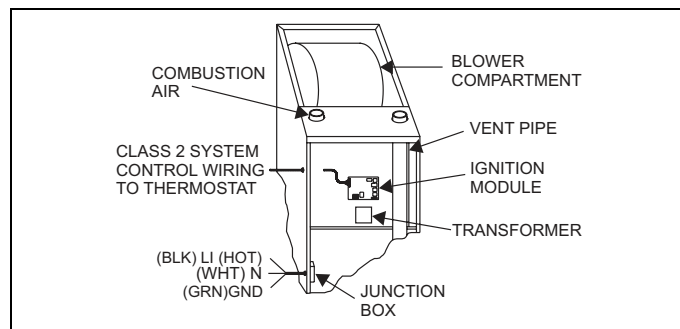
FIGURE 10: Electrical Wiring
