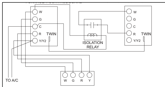
FIGURE 8: Single Stage Twinning Wiring Diagram
